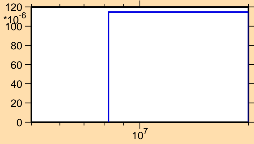
\sigma vs. E for ^{151}\text{Gd}(n,t)
