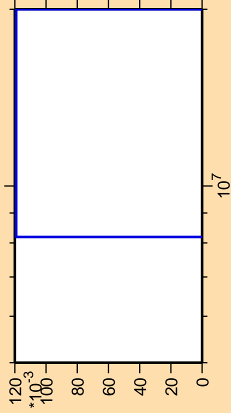
\Delta\sigma/\sigma vs. E for ^{151}\text{Gd}(n,3n\alpha)
