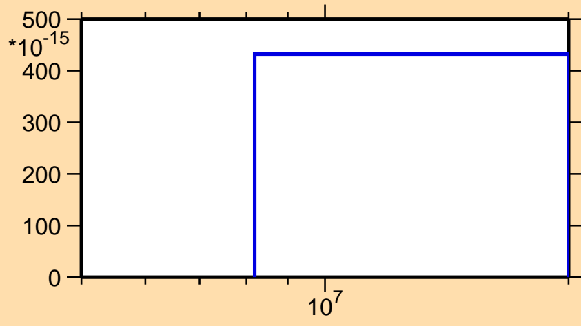
\sigma vs. E for ^{151}\text{Gd}(\text{mt117})
