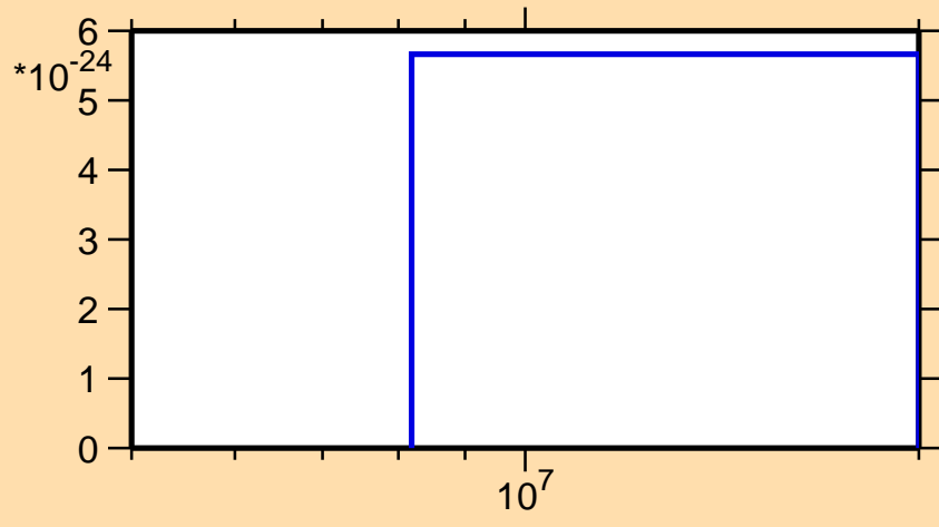
\sigma vs. E for ^{151}\text{Gd}(\text{mt } 11)
