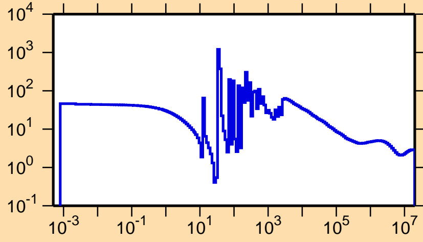
\sigma vs. E for ^{152}\text{Gd}(n,\text{el.})
