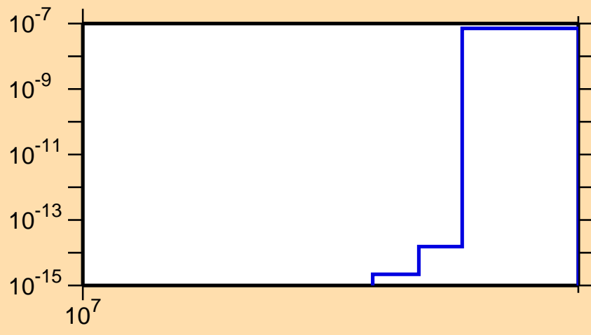
\sigma vs. E for ^{152}\text{Gd}(n,2np)
