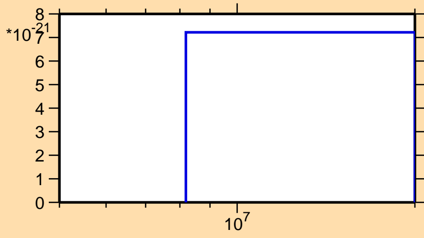
\sigma vs. E for ^{152}\text{Gd}(\text{mt } 11)
