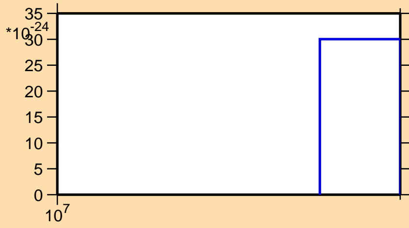
\sigma vs. E for ^{153}\text{Gd} (mt 11)
