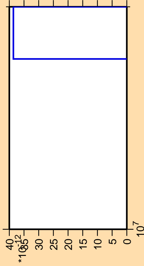
\Delta\sigma/\sigma vs. E for ^{153}\text{Gd} (mt 11)
