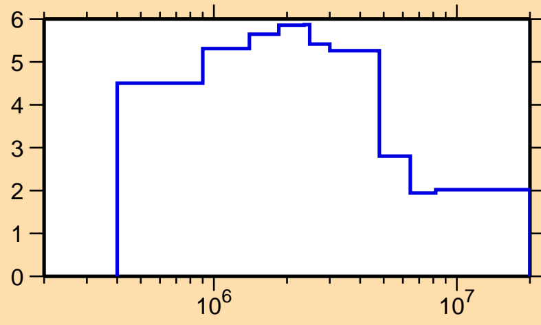
\Delta\sigma/\sigma vs. E for ^{153}\text{Gd}(n,\text{el.})
