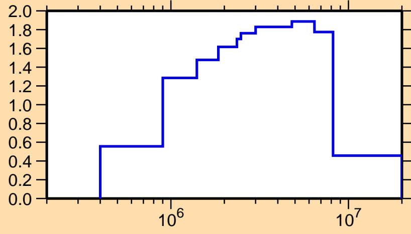
\sigma vs. E for ^{153}\text{Gd}(n,n\text{cont.})
