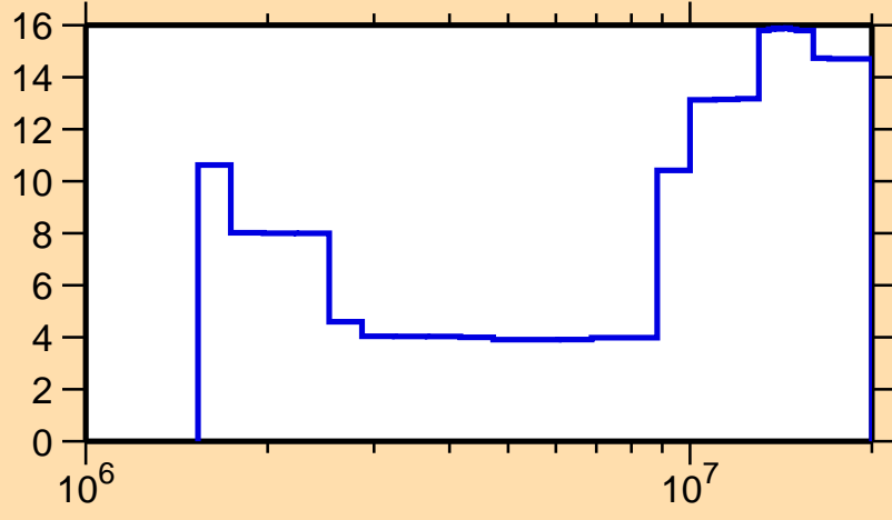
\Delta\sigma/\sigma vs. E for ^{154}\text{Gd}(n,ncont.)
