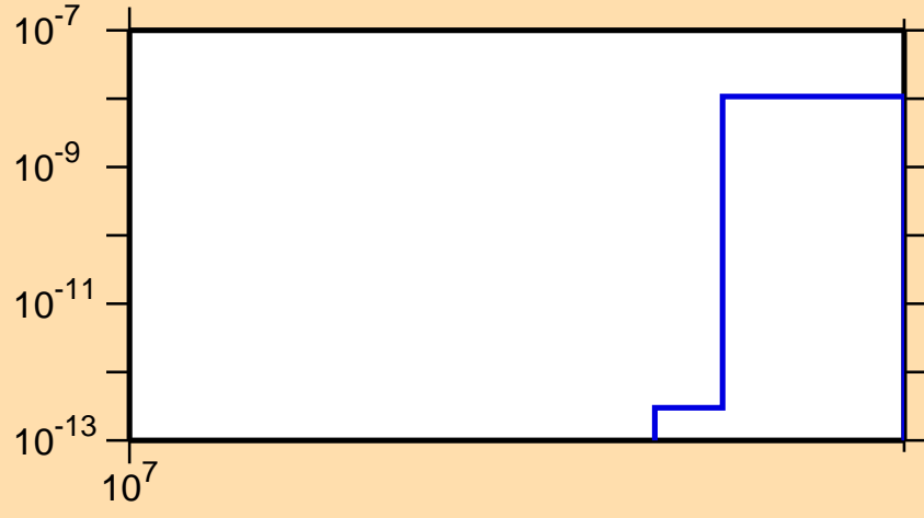
\sigma vs. E for ^{154}\text{Gd}(n,\text{nd})
