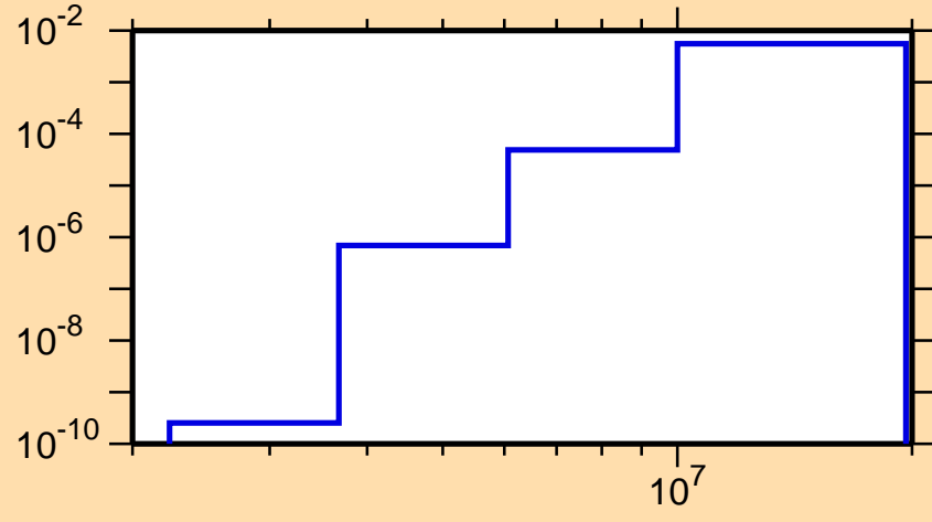
\sigma vs. E for ^{154}\text{Gd}(n,p)
