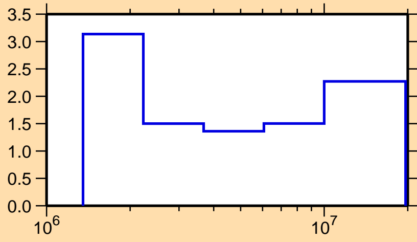
\Delta\sigma/\sigma vs. E for ^{154}\text{Gd}(n,n\text{onel.})
