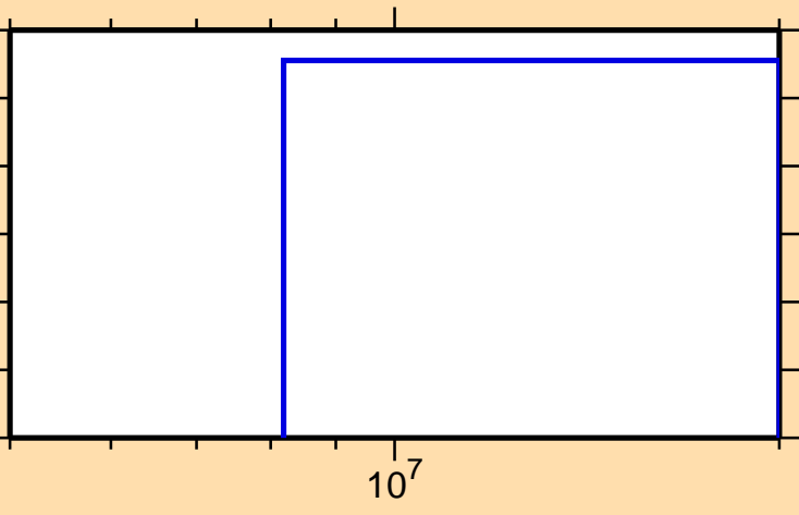
\sigma vs. E for ^{154}\text{Gd}(n,t)
