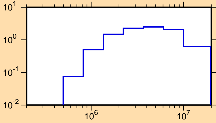
\sigma vs. E for ^{155}\text{Gd}(n,n\text{cont.})
