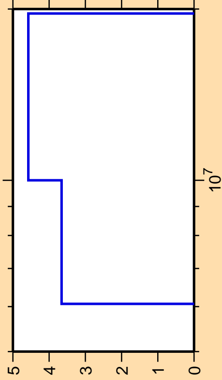
\Delta\sigma/\sigma vs. E for ^{155}\text{Gd}(n,n\text{cont.})
