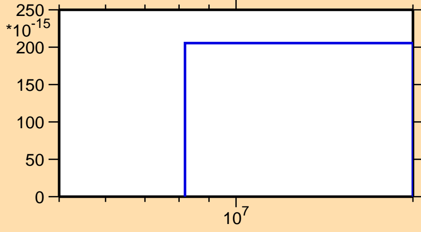
\sigma vs. E for ^{155}\text{Gd}(n,p\alpha)
