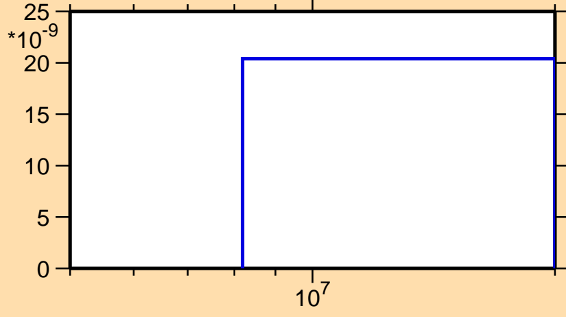
\sigma vs. E for ^{155}\text{Gd}(n,nd)
