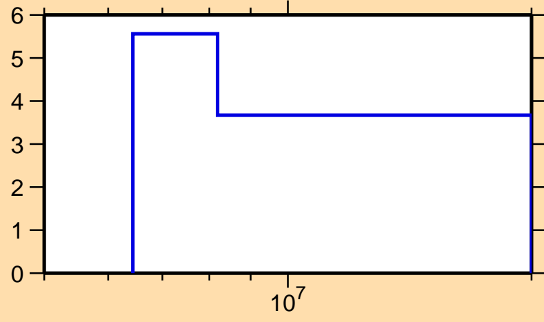
\Delta\sigma/\sigma vs. E for ^{155}\text{Gd}(n,2n)
