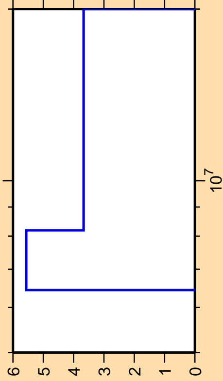
\Delta\sigma/\sigma vs. E for ^{155}\text{Gd}(n,2n)
