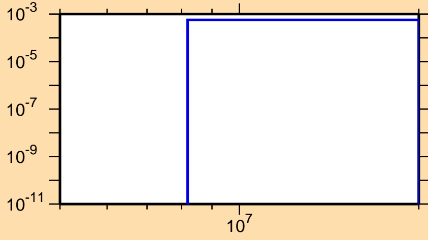
\sigma vs. E for ^{155}\text{Gd}(n,d)
