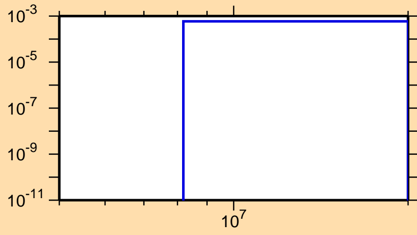
\sigma vs. E for ^{155}\text{Gd}(n,np)
