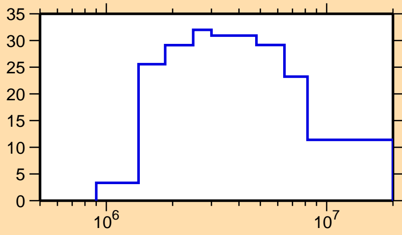
\Delta\sigma/\sigma vs. E for ^{155}\text{Gd}(n,p)
