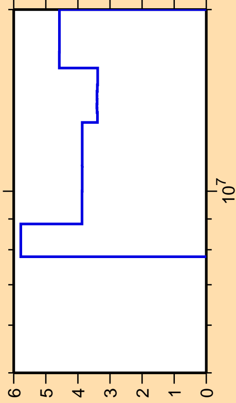
\Delta\sigma/\sigma vs. E for ^{156}\text{Gd}(n,2n)
