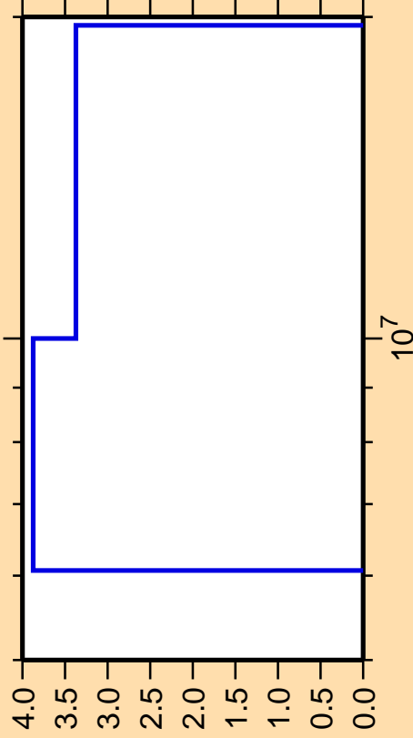
\Delta\sigma/\sigma vs. E for ^{156}\text{Gd}(n,2n)
