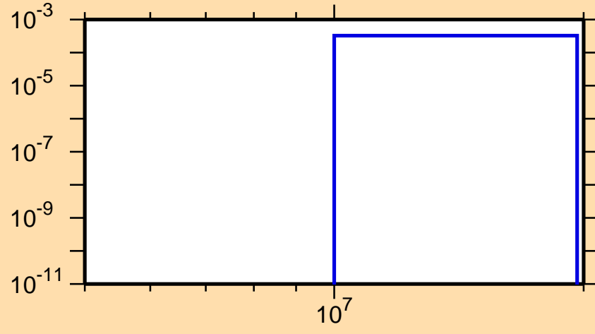
\sigma vs. E for ^{156}\text{Gd}(n,np)
