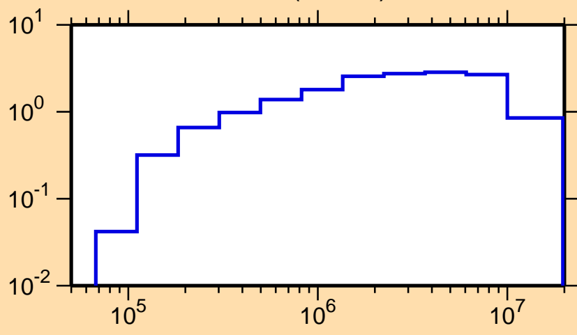
\sigma vs. E for ^{156}\text{Gd}(n,\text{inel.})
