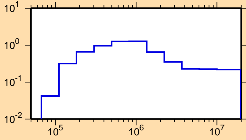
\sigma vs. E for ^{156}\text{Gd}(n,n_1)
