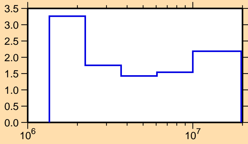
\Delta\sigma/\sigma vs. E for ^{156}\text{Gd}(n,n\text{onel.})
