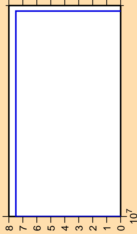
\Delta\sigma/\sigma vs. E for ^{156}\text{Gd}(n,3n)
