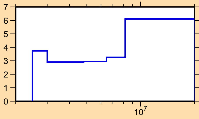
\Delta\sigma/\sigma vs. E for ^{156}\text{Gd}(n,n\text{cont.})
