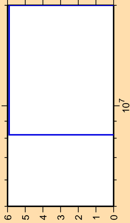
\Delta\sigma/\sigma vs. E for ^{156}\text{Gd}(n,2np)
