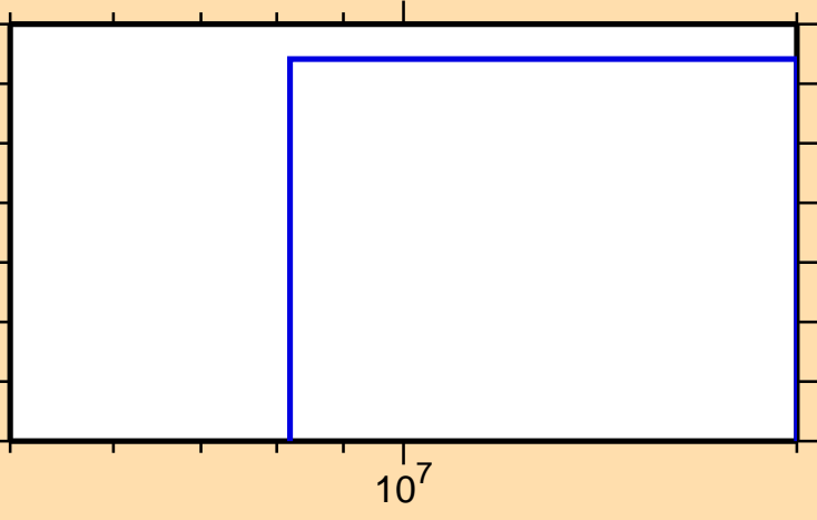
\sigma vs. E for ^{156}\text{Gd}(n,nt)
