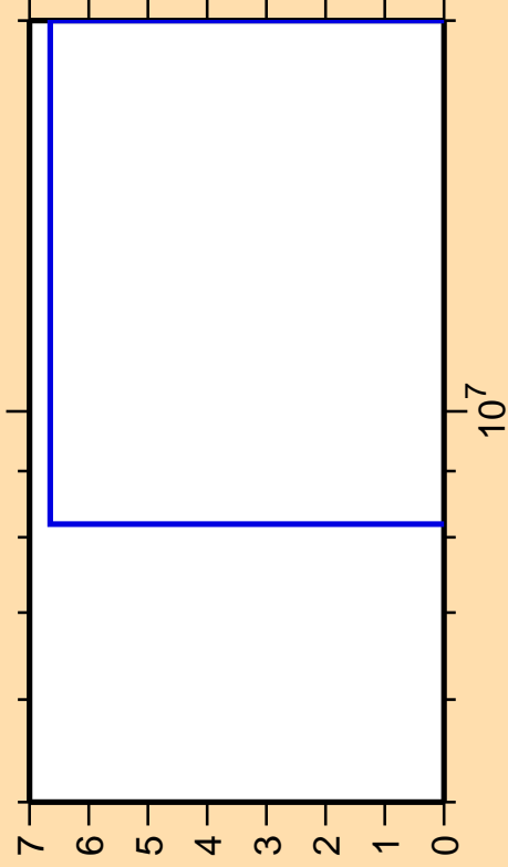
\Delta\sigma/\sigma vs. E for ^{156}\text{Gd}(n,\alpha)
