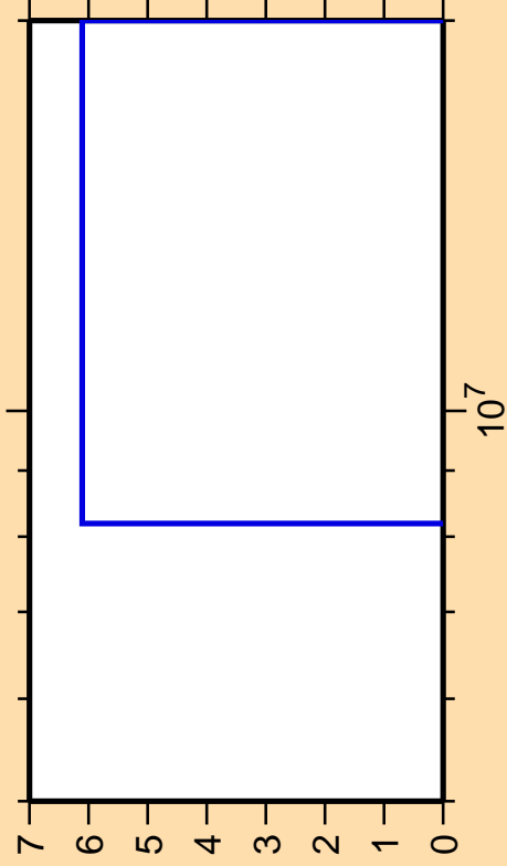
\Delta\sigma/\sigma vs. E for ^{156}\text{Gd}(n,n_{\text{cont}})
