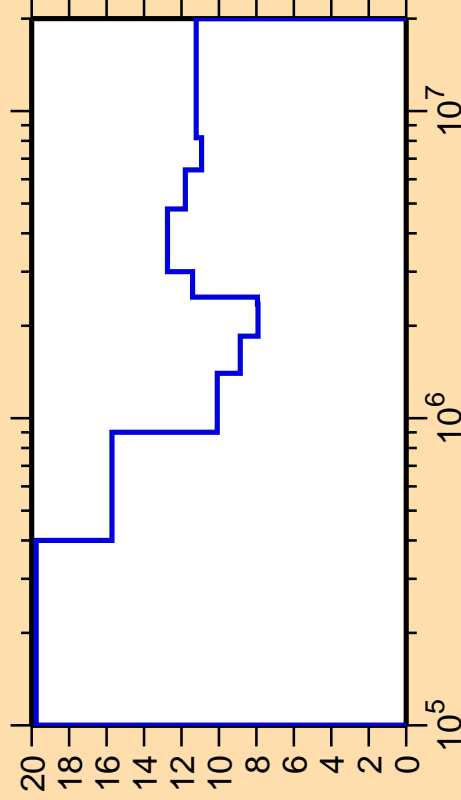
\Delta\sigma/\sigma vs. E for ^{156}\text{Gd}(n,n_2)
