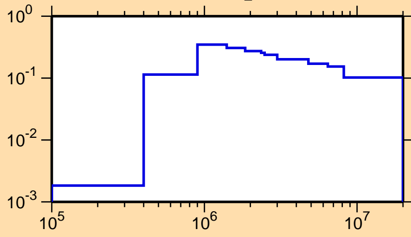
\sigma vs. E for ^{156}\text{Gd}(n,n_2)
