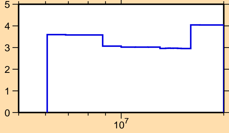
\Delta\sigma/\sigma vs. E for ^{157}\text{Gd}(n,2n)
