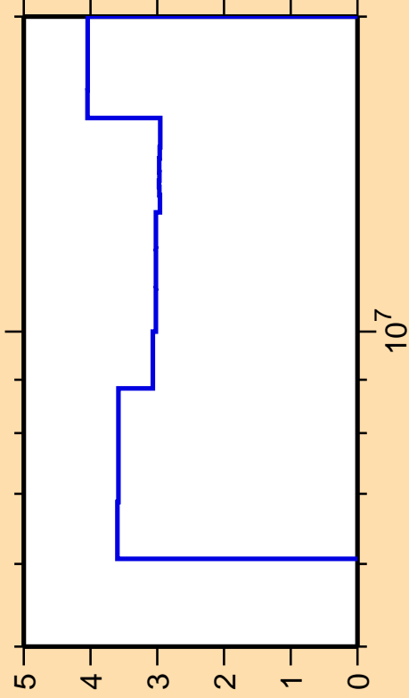
\Delta\sigma/\sigma vs. E for ^{157}\text{Gd}(n,2n)
