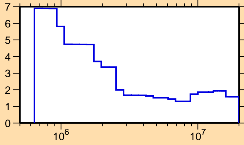
\Delta\sigma/\sigma vs. E for ^{157}\text{Gd}(n,n\text{onel.})
