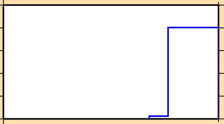
\sigma vs. E for ^{157}\text{Gd}(n,2np)
