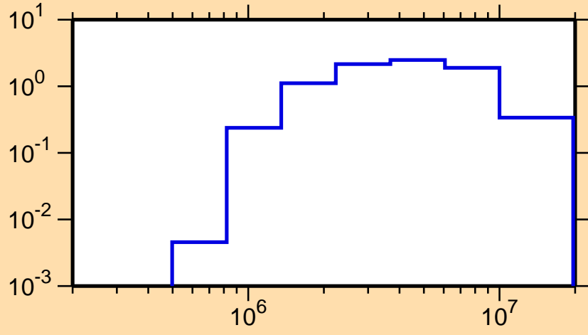
\sigma vs. E for ^{157}\text{Gd}(n,n\text{cont.})
