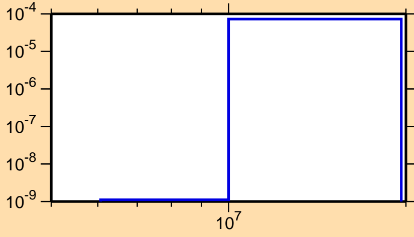
\sigma vs. E for ^{157}\text{Gd}(n,n\alpha)
