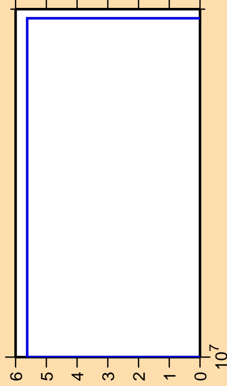
\Delta\sigma/\sigma vs. E for ^{157}\text{Gd}(n,3n)
