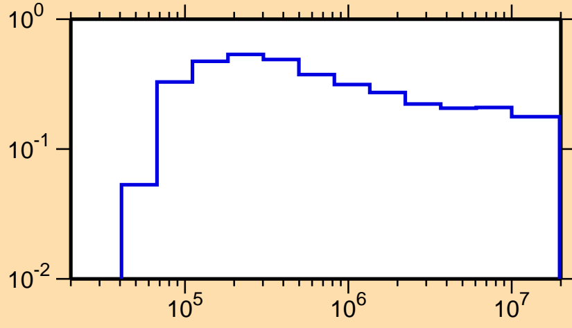
\sigma vs. E for ^{157}\text{Gd}(n,n_1)
