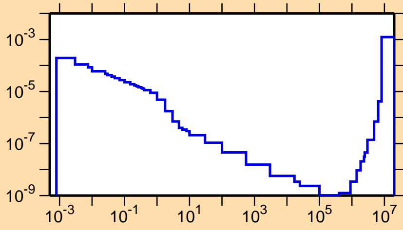
\sigma vs. E for ^{157}\text{Gd}(n,\alpha)
