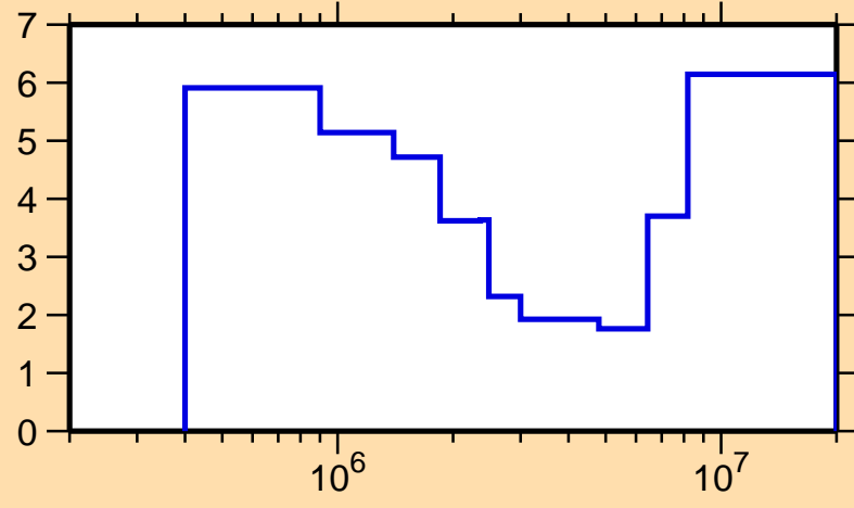
\Delta\sigma/\sigma vs. E for ^{157}\text{Gd}(n,\text{inel.})
