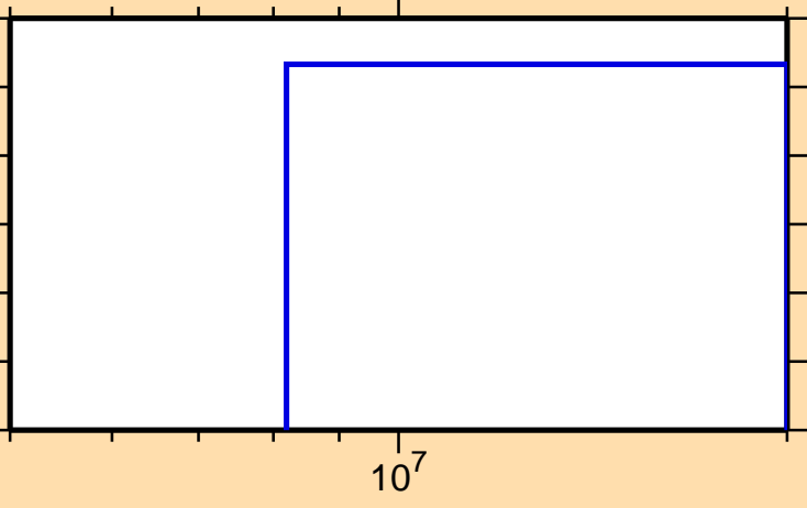
\sigma vs. E for ^{157}\text{Gd}(n,\text{nd})
