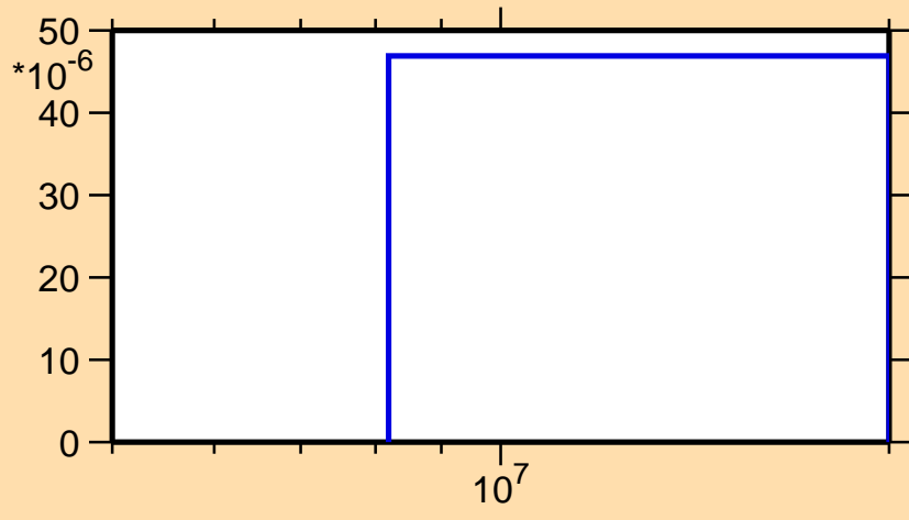
\sigma vs. E for ^{157}\text{Gd}(n,t)
