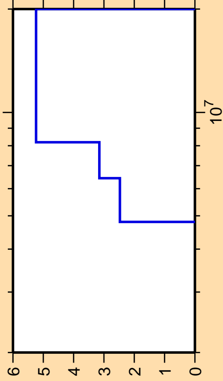
\Delta\sigma/\sigma vs. E for ^{157}\text{Gd}(n,n_{\text{cont}}) .
