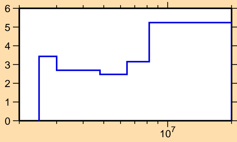
\Delta\sigma/\sigma vs. E for ^{157}\text{Gd}(n,n\text{cont.})
