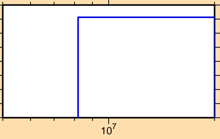
\sigma vs. E for ^{157}\text{Gd}(n,\text{He3})
