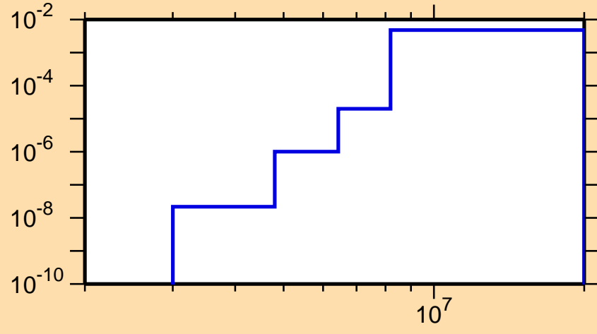
\sigma vs. E for ^{157}\text{Gd}(n,p)
