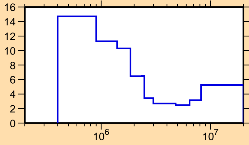
\Delta\sigma/\sigma vs. E for ^{157}\text{Gd}(n,ncont.)
