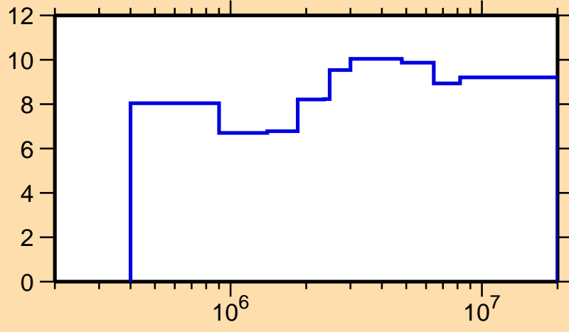
\Delta\sigma/\sigma vs. E for ^{157}\text{Gd}(n,n_1)
