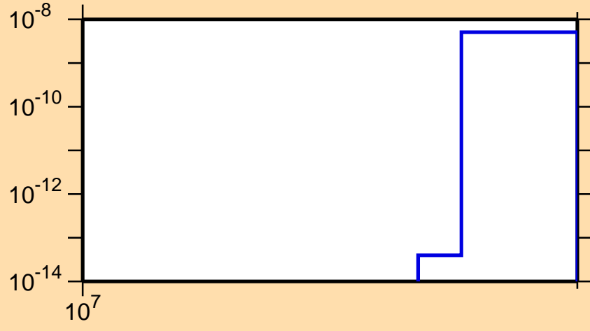
\sigma vs. E for ^{158}\text{Gd}(n,nt)
