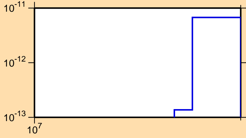
\sigma vs. E for ^{158}\text{Gd}(n,\text{He}3)
