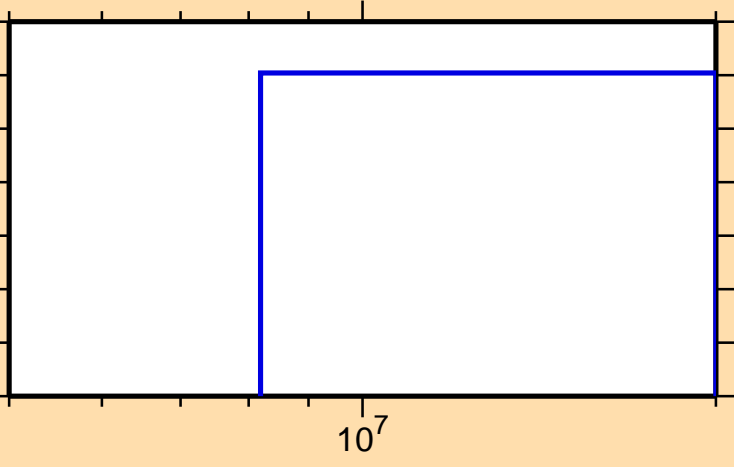
\sigma vs. E for ^{158}\text{Gd}(n,\text{He3})
