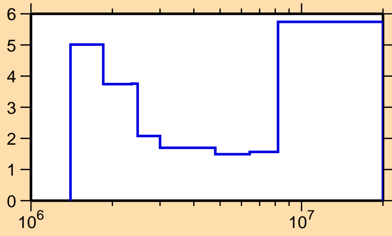
\Delta\sigma/\sigma vs. E for ^{158}\text{Gd}(n,\text{inel.})
