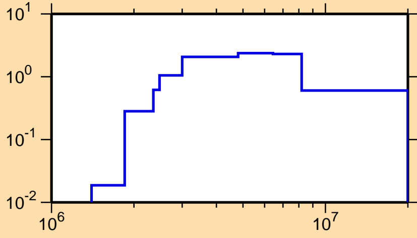
\sigma vs. E for ^{158}\text{Gd}(n,n\text{cont.})
