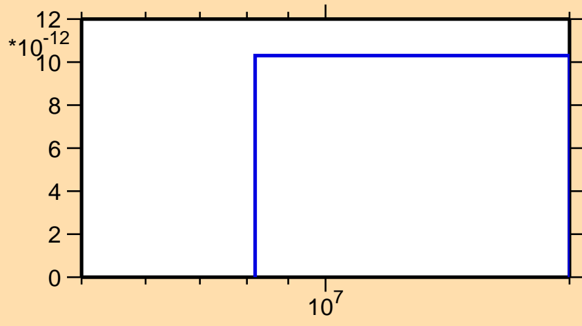
\sigma vs. E for ^{158}\text{Gd}(n,2np)
