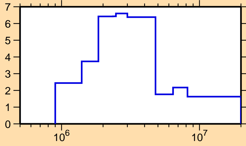
\Delta\sigma/\sigma vs. E for ^{158}\text{Gd}(n,\text{el.})
