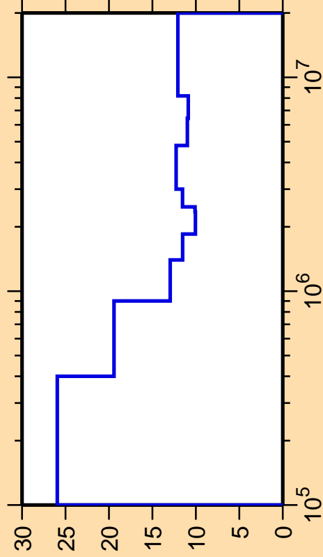
\Delta\sigma/\sigma vs. E for ^{158}\text{Gd}(n,n_2)
