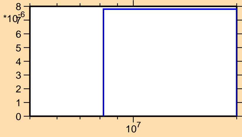
\sigma vs. E for ^{158}\text{Gd}(n,t)
