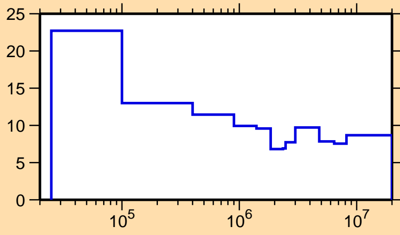
\Delta\sigma/\sigma vs. E for ^{158}\text{Gd}(n,n_1)
