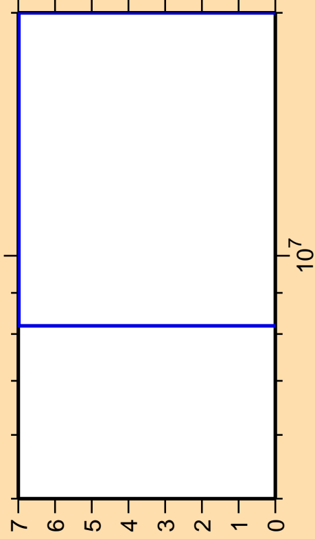
\Delta\sigma/\sigma vs. E for ^{158}\text{Gd}(n,2np)
