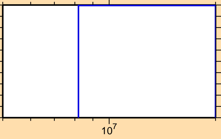
\sigma vs. E for ^{158}\text{Gd}(n,\text{nd})
