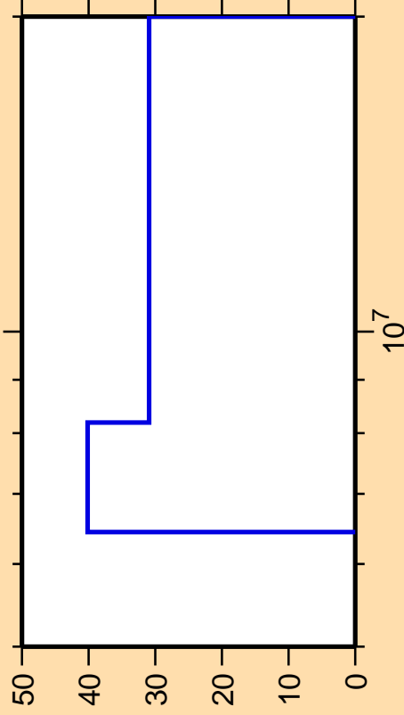
\Delta\sigma/\sigma vs. E for ^{158}\text{Gd}(n,\gamma)
