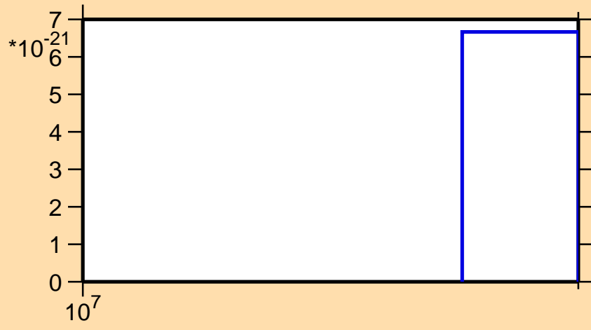
\sigma vs. E for ^{159}\text{Gd} (mt 11)
