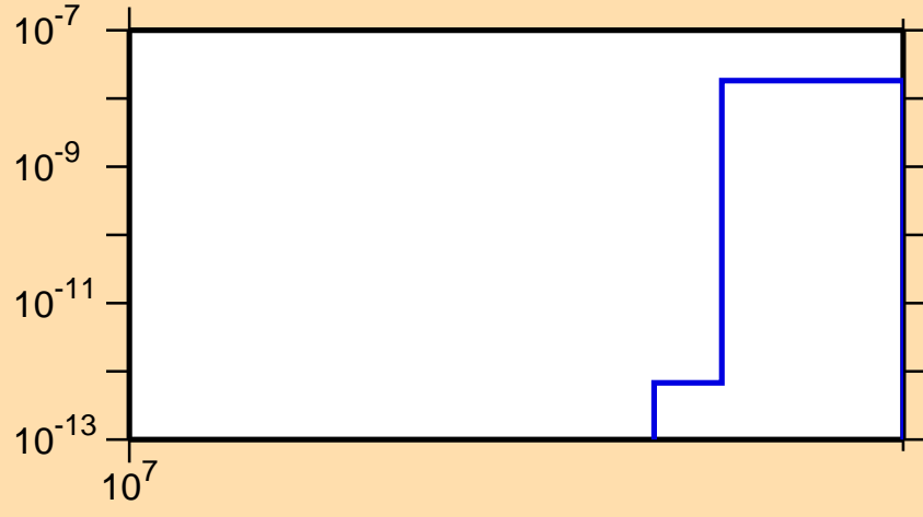
\sigma vs. E for ^{159}\text{Gd}(n,nt)
