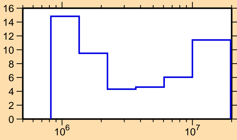
\Delta\sigma/\sigma vs. E for ^{159}\text{Gd}(n,n\text{cont.})
