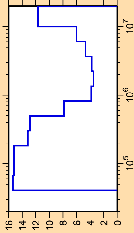
\Delta\sigma/\sigma vs. E for ^{159}\text{Gd}(n,\text{inel.})
