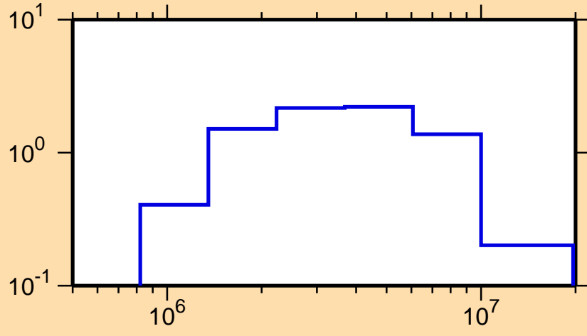
\sigma vs. E for ^{159}\text{Gd}(n,n\text{cont.})
