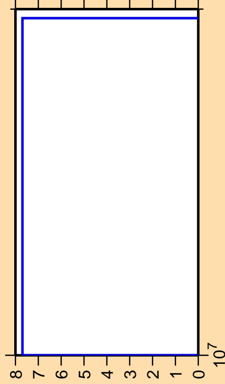
\Delta\sigma/\sigma vs. E for ^{159}\text{Gd}(n,3n)
