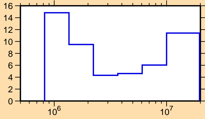
\Delta\sigma/\sigma vs. E for ^{159}\text{Gd}(n,n\text{cont.})
