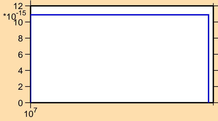
\sigma vs. E for ^{159}\text{Gd}(n,\text{He}3)
