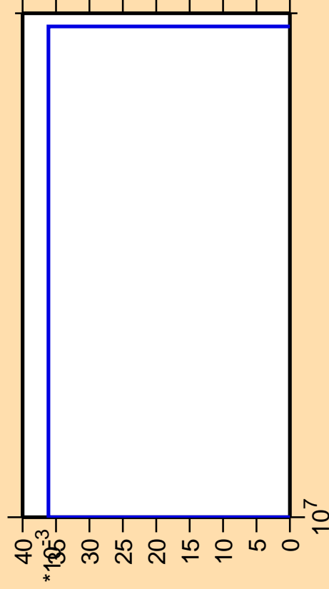
\Delta\sigma/\sigma vs. E for ^{159}\text{Gd}(n,\text{He}3)
