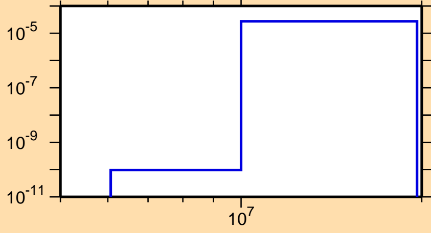
\sigma vs. E for ^{159}\text{Gd}(n,n\alpha)
