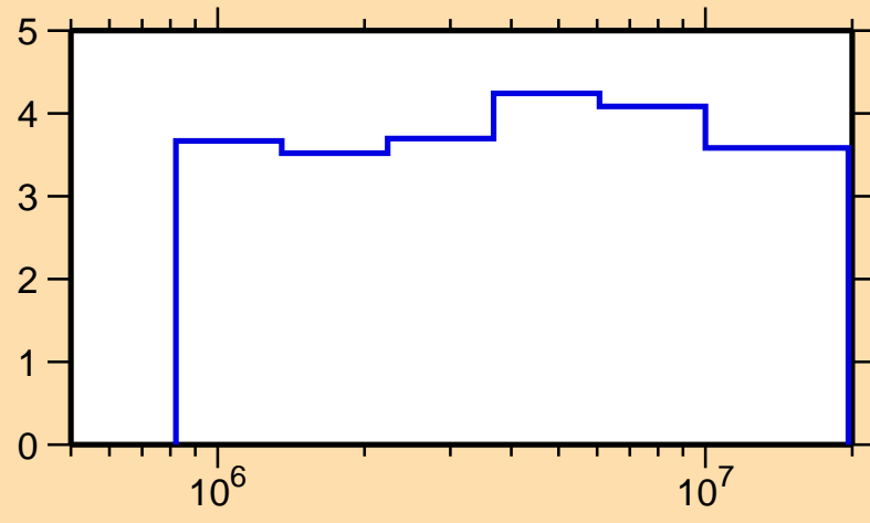
\Delta\sigma/\sigma vs. E for ^{159}\text{Gd}(n,n\text{onel.})
