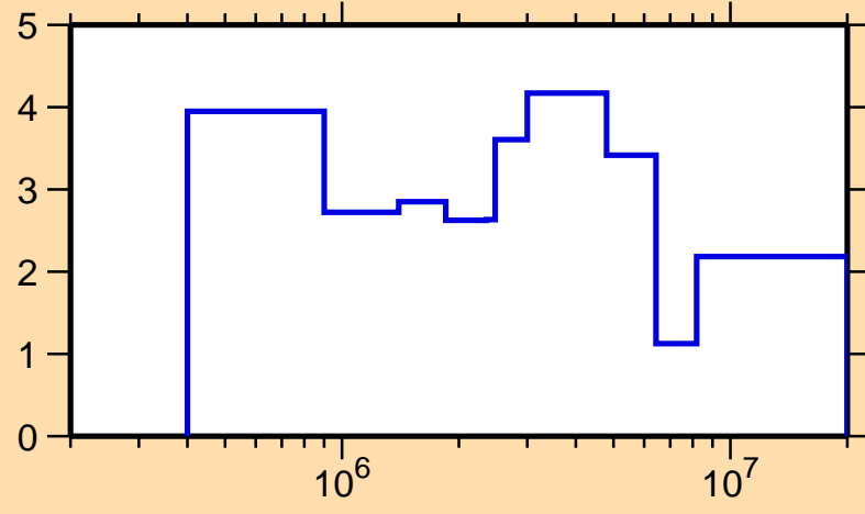
\Delta\sigma/\sigma vs. E for ^{159}\text{Gd}(n,\text{el.})
