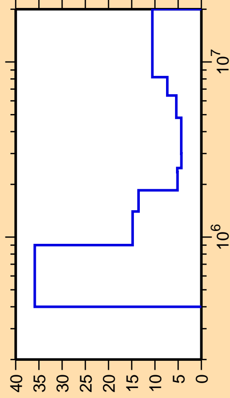
\Delta\sigma/\sigma vs. E for ^{159}\text{Gd}(n,\text{ncont.})
