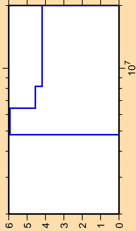
\Delta\sigma/\sigma vs. E for ^{159}\text{Gd}(n,2n)
