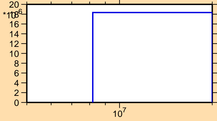
\sigma vs. E for ^{159}\text{Gd}(n,t)
