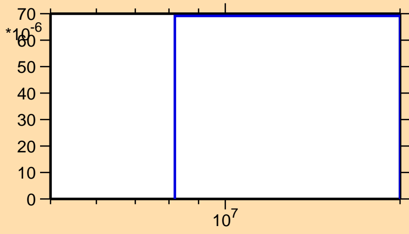
\sigma vs. E for ^{159}\text{Gd}(n,np)
