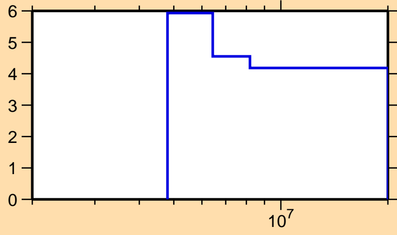
\Delta\sigma/\sigma vs. E for ^{159}\text{Gd}(n,2n)
