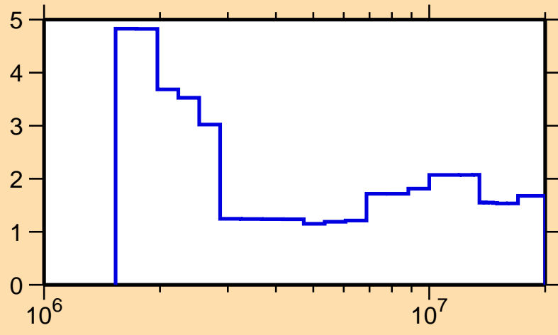
\Delta\sigma/\sigma vs. E for ^{160}\text{Gd}(n,n\text{onel.})
