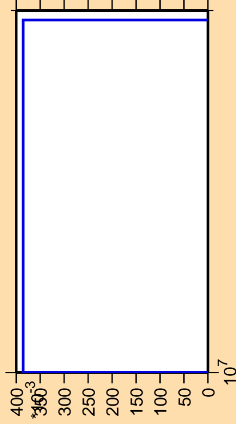
\Delta\sigma/\sigma vs. E for ^{160}\text{Gd}(n,2np)
