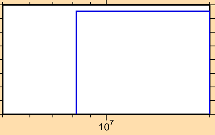
\sigma vs. E for ^{161}\text{Gd}(n,2np)
