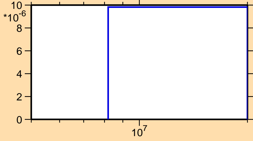
\sigma vs. E for ^{161}\text{Gd}(n,t)
