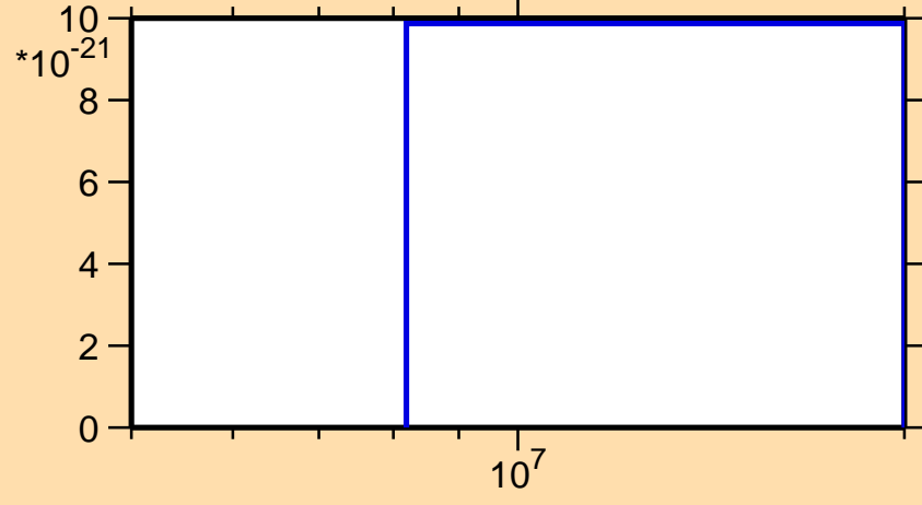
\sigma vs. E for ^{161}\text{Gd} (mt 11)
