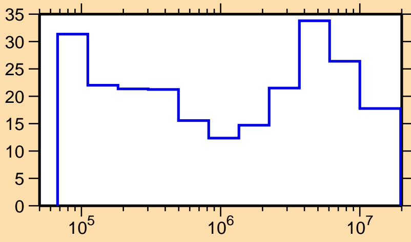
\Delta\sigma/\sigma vs. E for ^{162}\text{Gd}(n,n_1)
