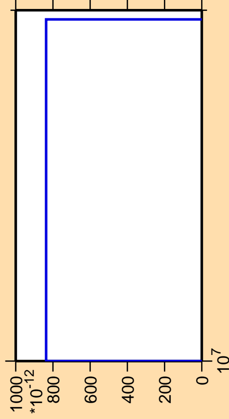
\Delta\sigma/\sigma vs. E for ^{162}\text{Gd} (mt 11)
