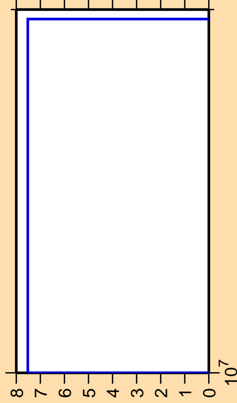
\Delta\sigma/\sigma vs. E for ^{162}\text{Gd}(n,3n)
