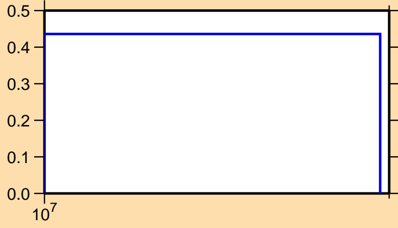
\sigma vs. E for ^{162}\text{Gd}(n,3n)
