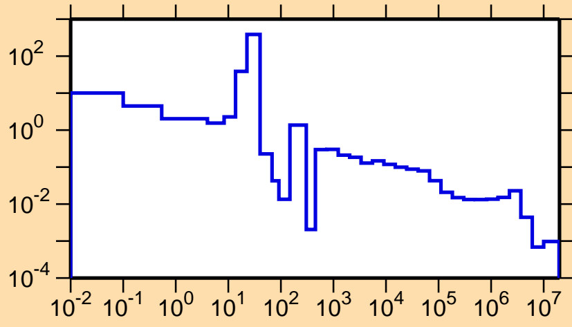
\sigma vs. E for ^{162}\text{Gd}(n,\gamma)
