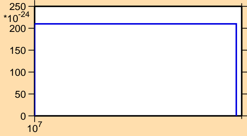
\sigma vs. E for ^{162}\text{Gd} (mt 11)
