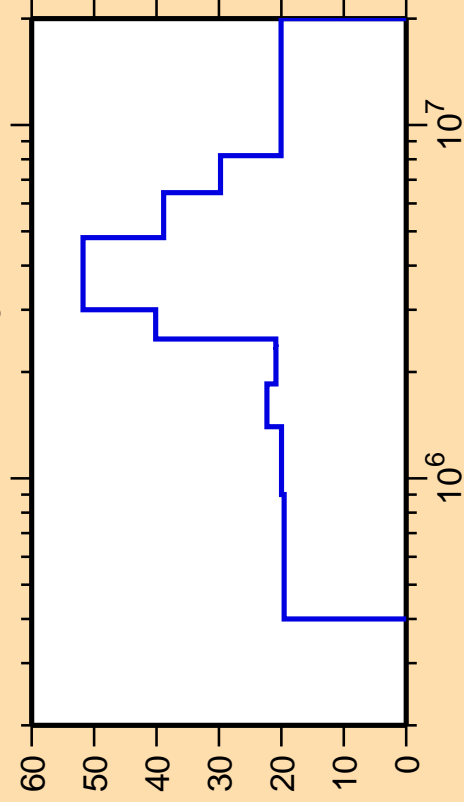
\Delta\sigma/\sigma vs. E for ^{162}\text{Gd}(n,n_3)
