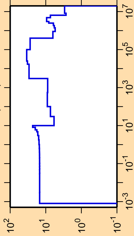
\Delta\sigma/\sigma vs. E for ^{162}\text{Gd}(n,\text{el.})
