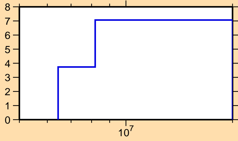
\Delta\sigma/\sigma vs. E for ^{162}\text{Gd}(n,2n)
