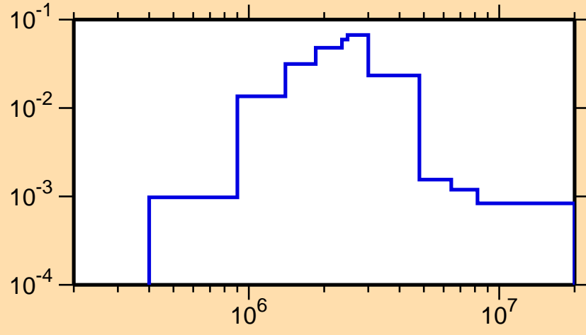
\sigma vs. E for ^{162}\text{Gd}(n,n_3)
