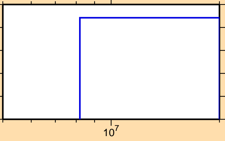
\sigma vs. E for ^{162}\text{Gd}(\text{mt } 11)
