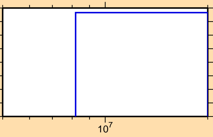
\sigma vs. E for ^{162}\text{Gd}(n,n\alpha)
