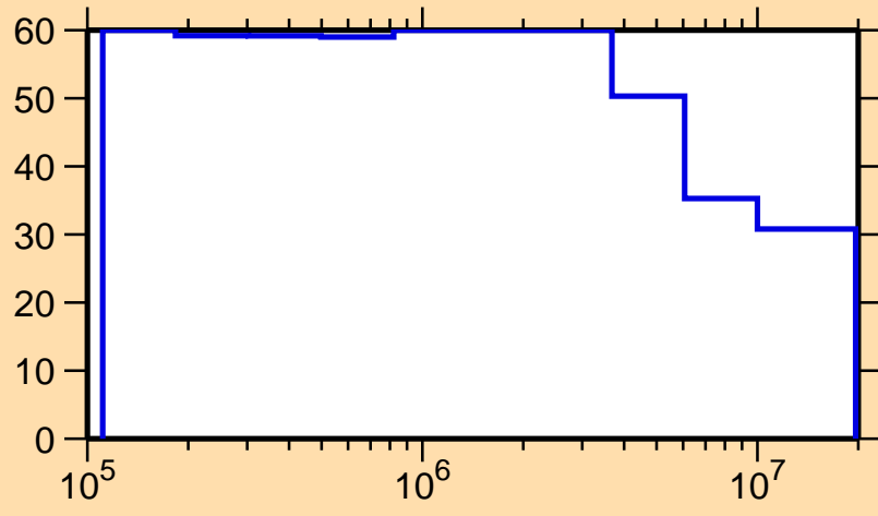
\Delta\sigma/\sigma vs. E for ^{163}\text{Gd}(n,n_1)
