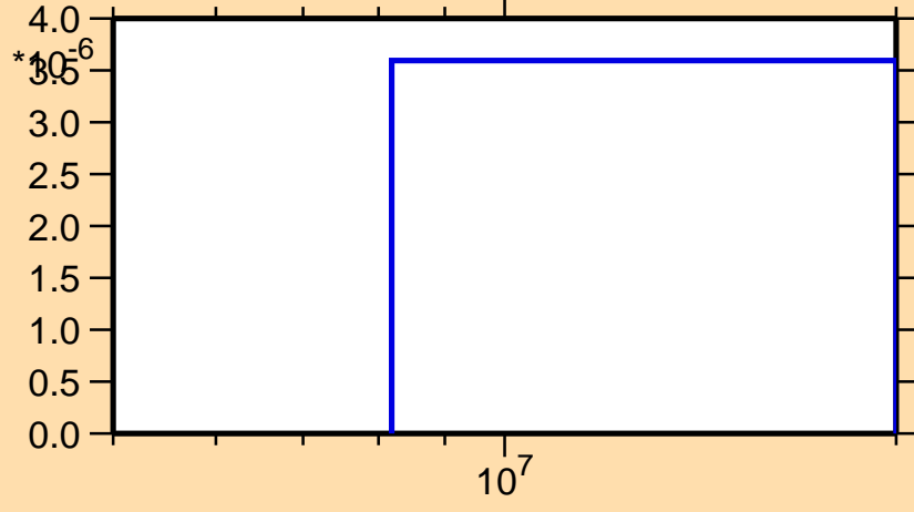
\sigma vs. E for ^{163}\text{Gd}(n,n\alpha)
