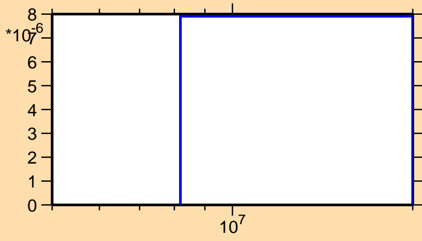
\sigma vs. E for ^{163}\text{Gd}(n,np)
