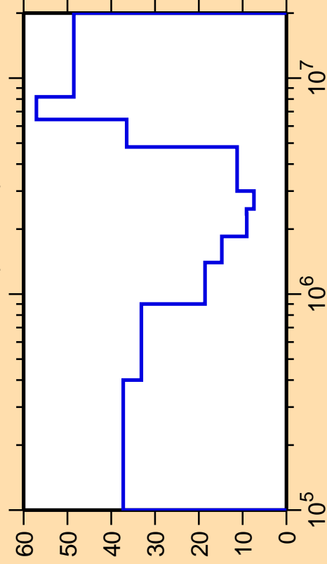
\Delta\sigma/\sigma vs. E for ^{163}\text{Gd}(n,\text{inel.})
