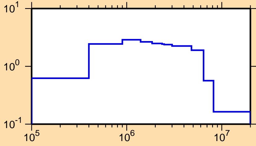
\sigma vs. E for ^{163}\text{Gd}(n,\text{inel.})
