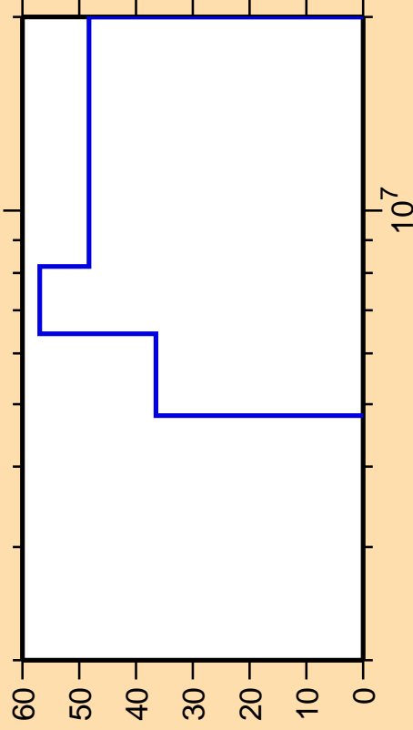
\Delta\sigma/\sigma vs. E for ^{163}\text{Gd}(n,n\text{cont.})
