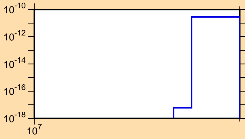
\sigma vs. E for ^{164}\text{Gd}(n,2np)
