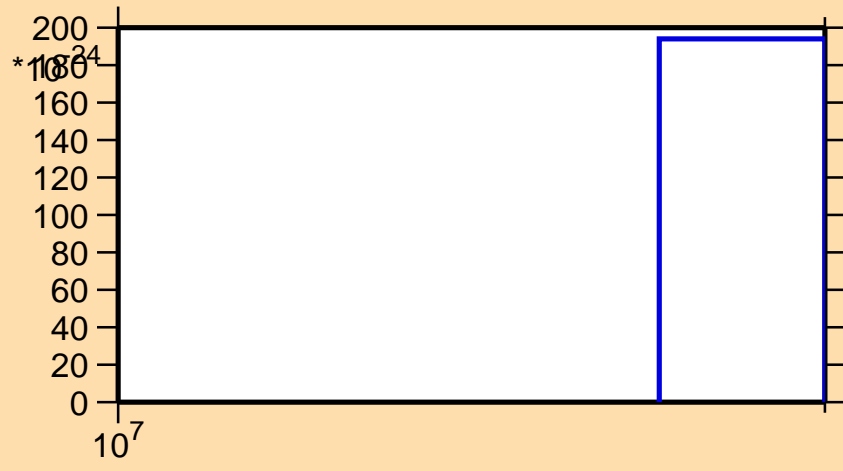
\sigma vs. E for ^{164}\text{Gd} (mt 11)
