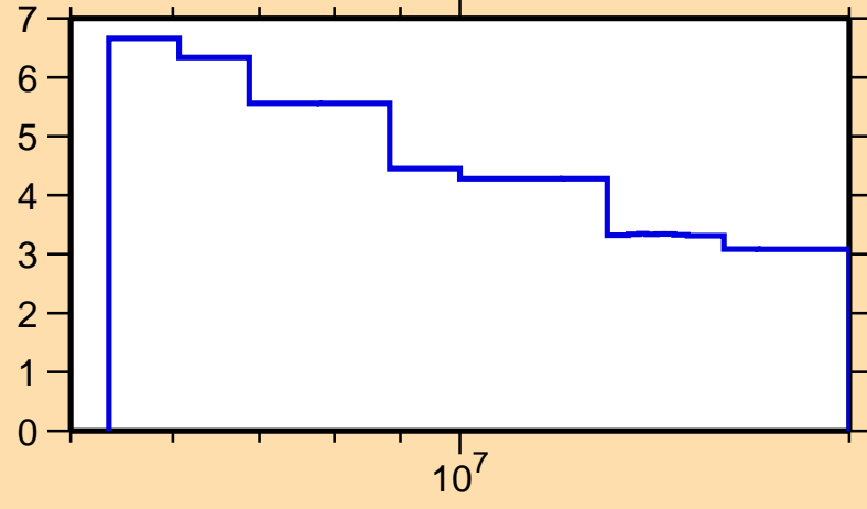
\Delta\sigma/\sigma vs. E for ^{164}\text{Gd}(n,\text{nonel.})
