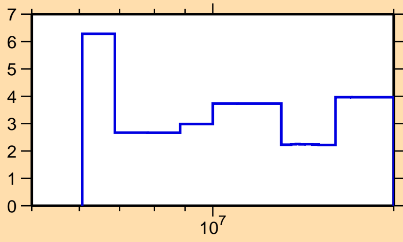
\Delta\sigma/\sigma vs. E for ^{164}\text{Gd}(n,\text{tot.})
