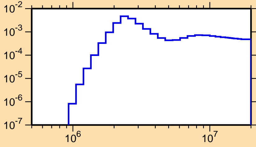
\sigma vs. E for ^{164}\text{Gd}(n,n_4)
