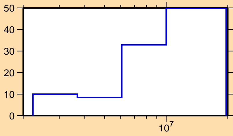
\Delta\sigma/\sigma vs. E for ^{164}\text{Gd}(n,n\text{cont.})
