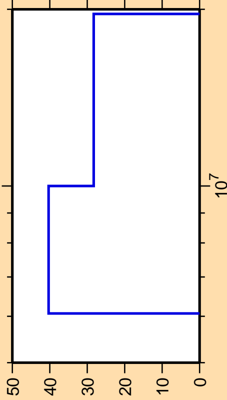
\Delta\sigma/\sigma vs. E for ^{164}\text{Gd}(n,n_1)
