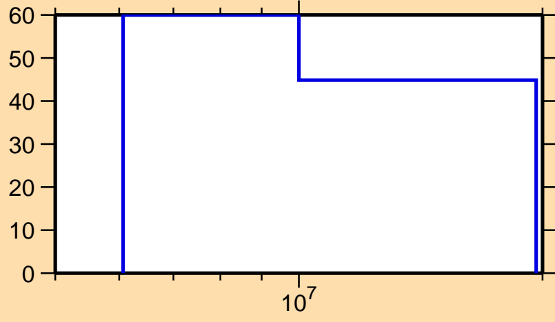
\Delta\sigma/\sigma vs. E for ^{164}\text{Gd}(n,p)
