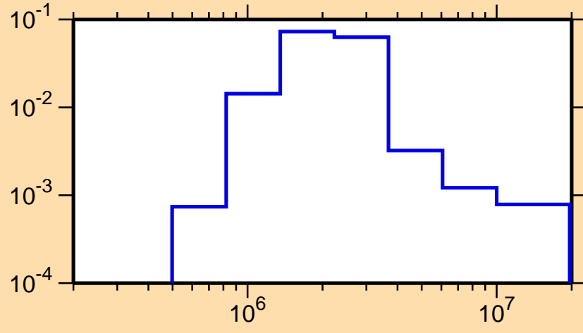
\sigma vs. E for ^{164}\text{Gd}(n,n_3)
