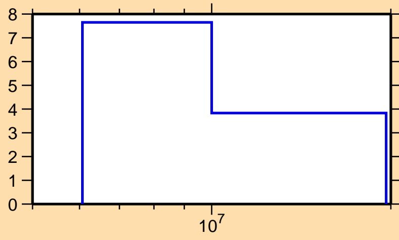
\Delta\sigma/\sigma vs. E for ^{164}\text{Gd}(n,\text{el.})
