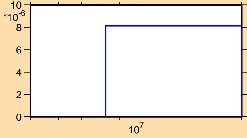
\sigma vs. E for ^{164}\text{Gd}(n,d)
