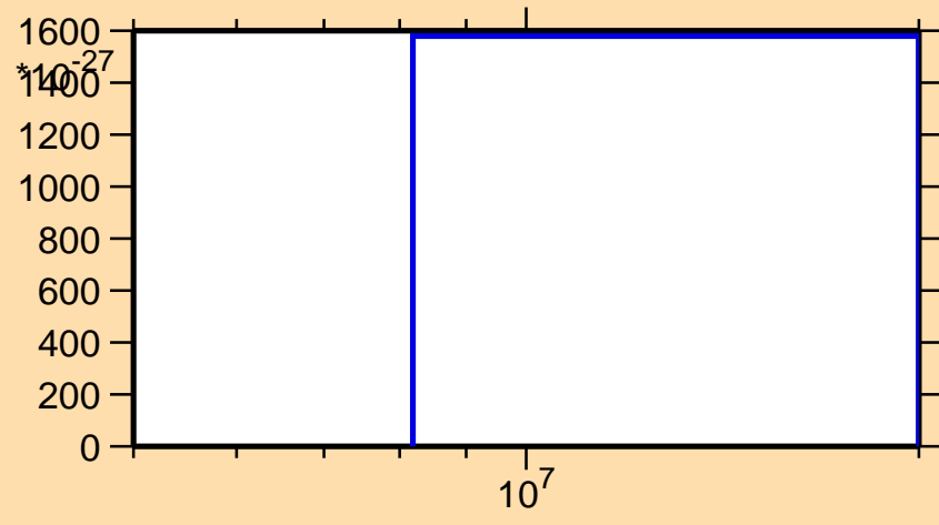
\sigma vs. E for ^{164}\text{Gd}(\text{mt } 11)
