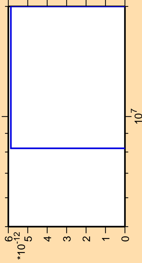
\Delta\sigma/\sigma vs. E for ^{164}\text{Gd}(\text{mt } 11)
