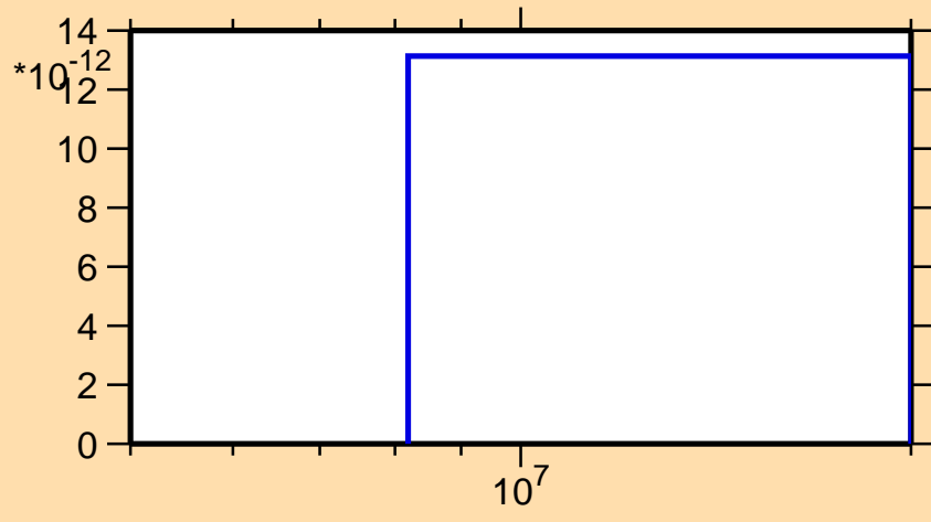
\sigma vs. E for ^{164}\text{Gd}(n,2n\alpha)
