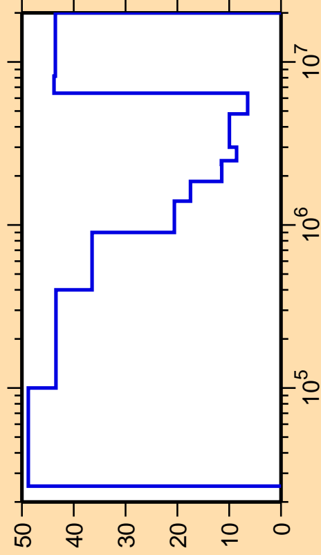
\Delta\sigma/\sigma vs. E for ^{164}\text{Gd}(n,\text{inel.})
