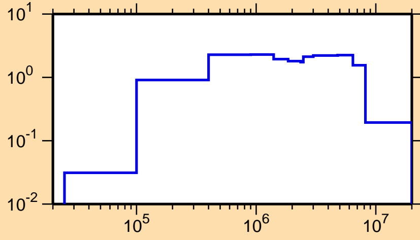
\sigma vs. E for ^{164}\text{Gd}(n,\text{inel.})
