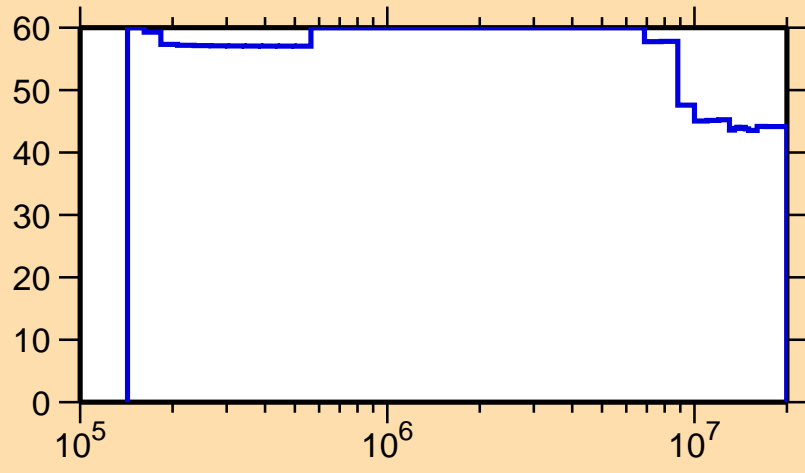
\Delta\sigma/\sigma vs. E for ^{165}\text{Gd}(n,n_1)
