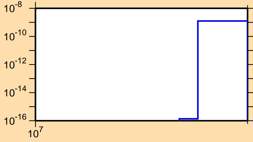
\sigma vs. E for ^{165}\text{Gd}(n,2np)
