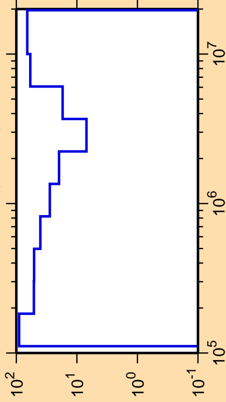
\Delta\sigma/\sigma vs. E for ^{165}\text{Gd}(n,\text{inel.})
