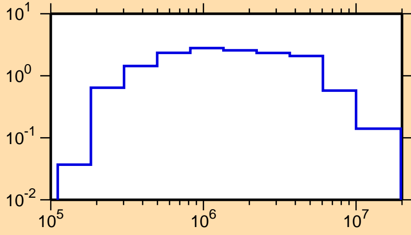
\sigma vs. E for ^{165}\text{Gd}(n,\text{inel.})
