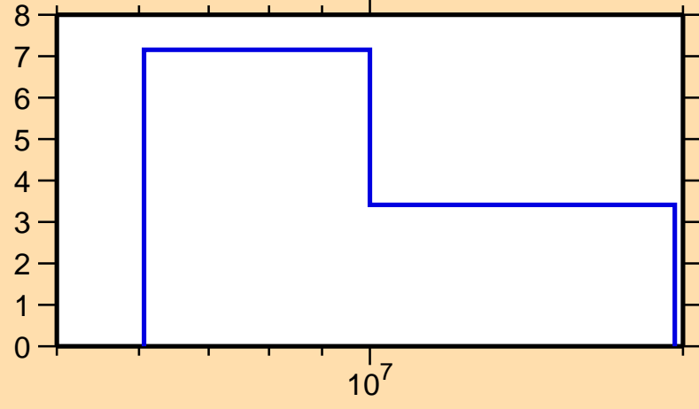
\Delta\sigma/\sigma vs. E for ^{165}\text{Gd}(n,\text{tot.})
