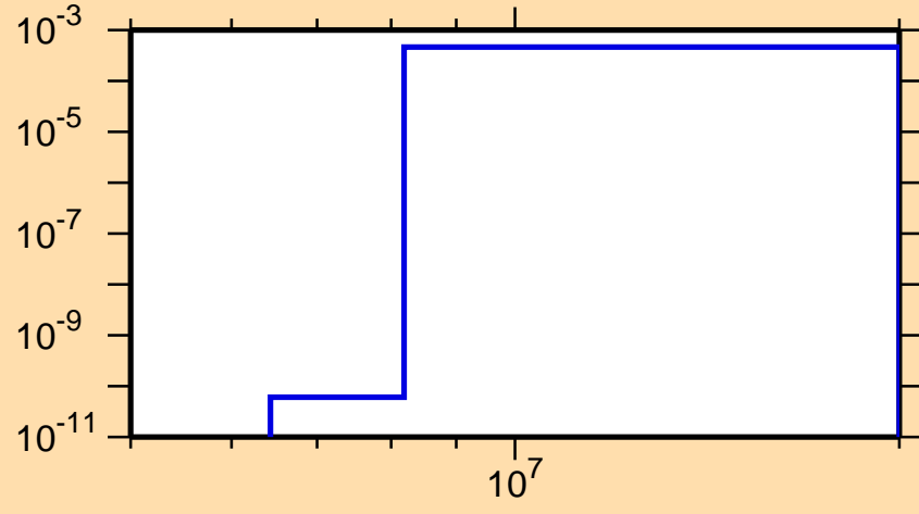
\sigma vs. E for ^{165}\text{Gd}(n,p)
