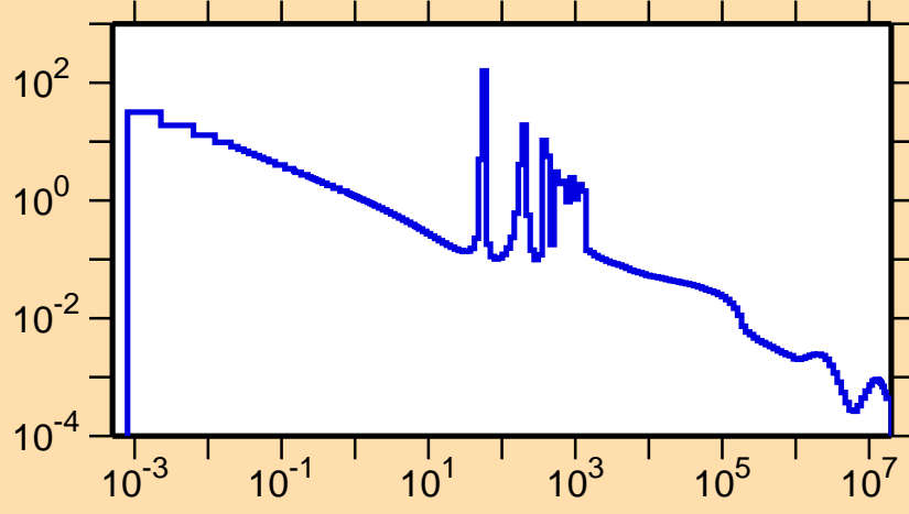
\sigma vs. E for ^{166}\text{Gd}(n,\gamma)
