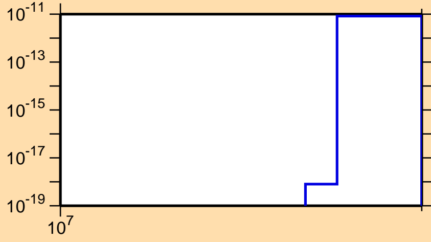
\sigma vs. E for ^{166}\text{Gd}(n,2np)
