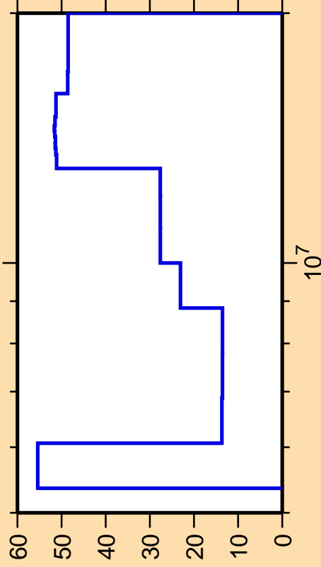
\Delta\sigma/\sigma vs. E for ^{166}\text{Gd}(n,2n)
