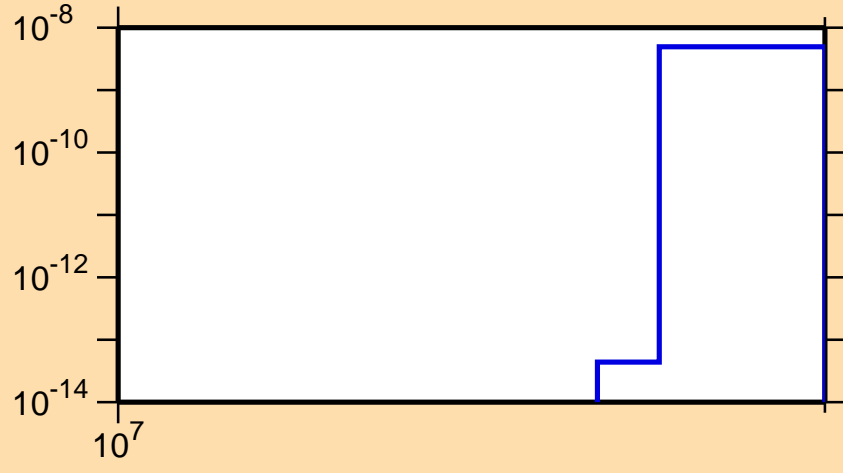
\sigma vs. E for ^{166}\text{Gd}(n,\text{nd})
