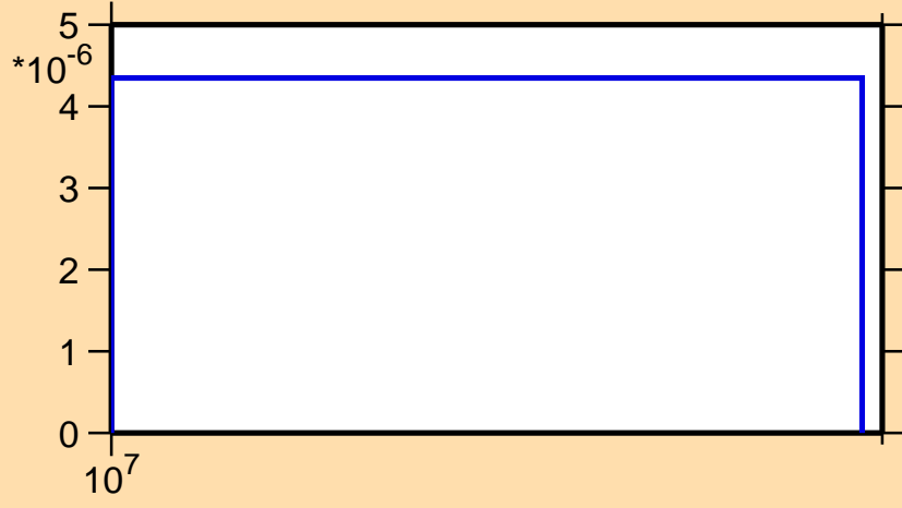
\sigma vs. E for ^{166}\text{Gd}(n,d)
