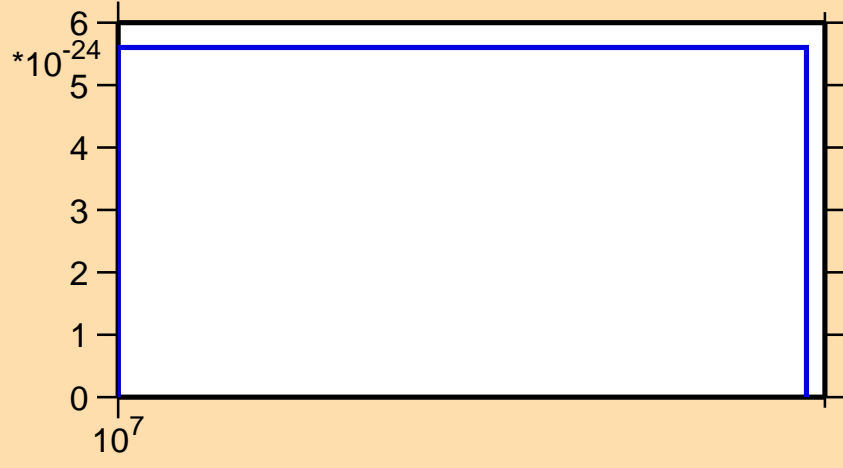
\sigma vs. E for ^{166}\text{Gd} (mt 11)
