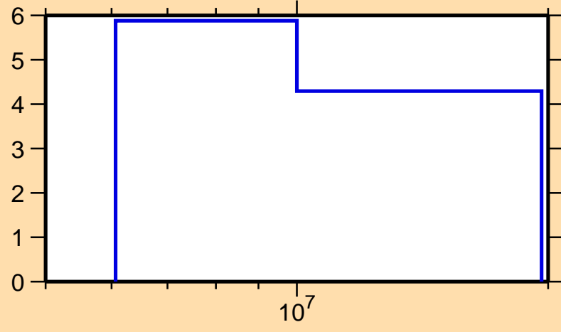
\Delta\sigma/\sigma vs. E for ^{166}\text{Gd}(n,\text{tot.})
