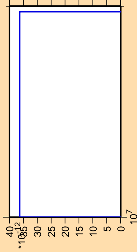
\Delta\sigma/\sigma vs. E for ^{166}\text{Gd} (mt 11)
