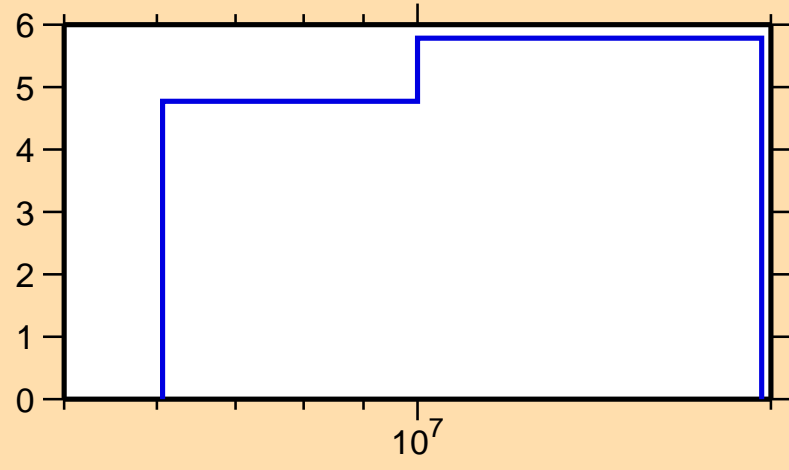
\Delta\sigma/\sigma vs. E for ^{166}\text{Gd}(n,\text{nonel.})
