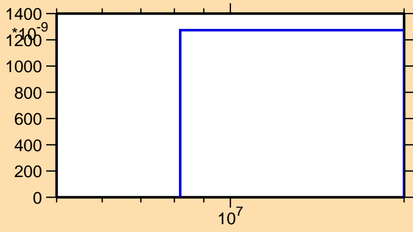
\sigma vs. E for ^{166}\text{Gd}(n,np)
