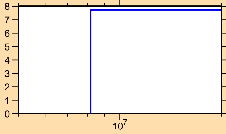
\Delta\sigma/\sigma vs. E for ^{166}\text{Gd}(n,\text{el.})
