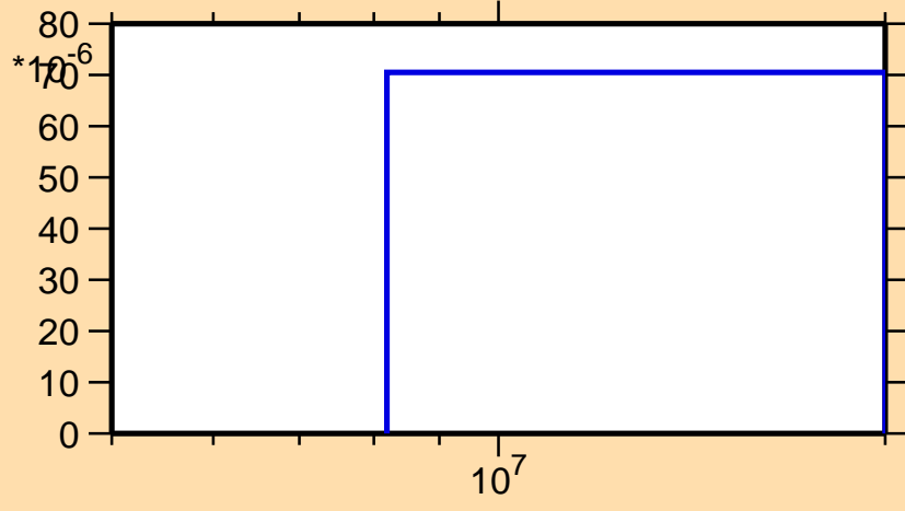
\sigma vs. E for ^{166}\text{Gd}(n,p)
