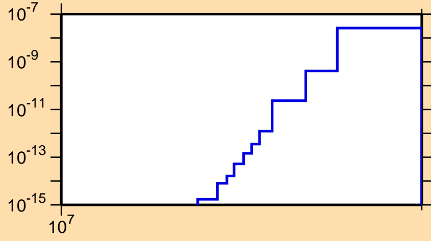
\sigma vs. E for ^{169}\text{Gd}(n,2n\alpha)
