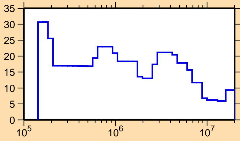
\Delta\sigma/\sigma vs. E for ^{169}\text{Gd}(n,\text{tot.})
