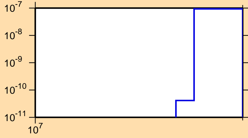
\sigma vs. E for ^{169}\text{Gd}(n,\text{nd})
