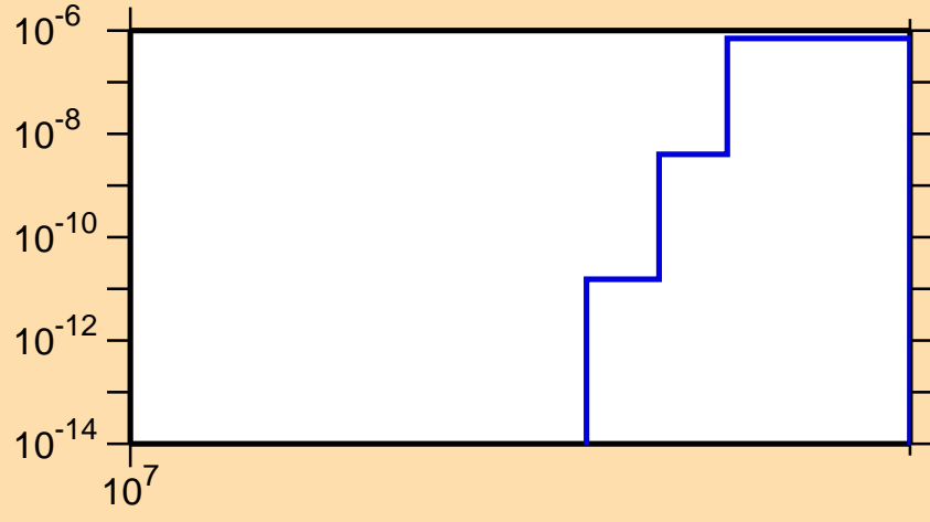
\sigma vs. E for ^{169}\text{Gd}(n,nt)
