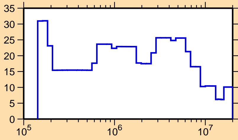
\Delta\sigma/\sigma vs. E for ^{169}\text{Gd}(n,\text{el.})
