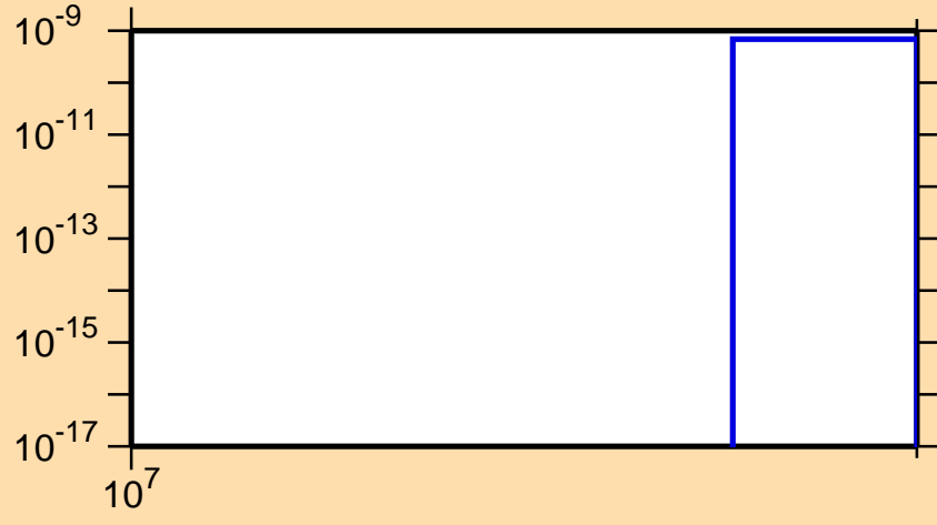
\sigma vs. E for ^{169}\text{Gd}(n,2np)
