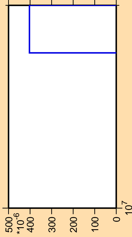
\Delta\sigma/\sigma vs. E for ^{169}\text{Gd} (mt 11)
