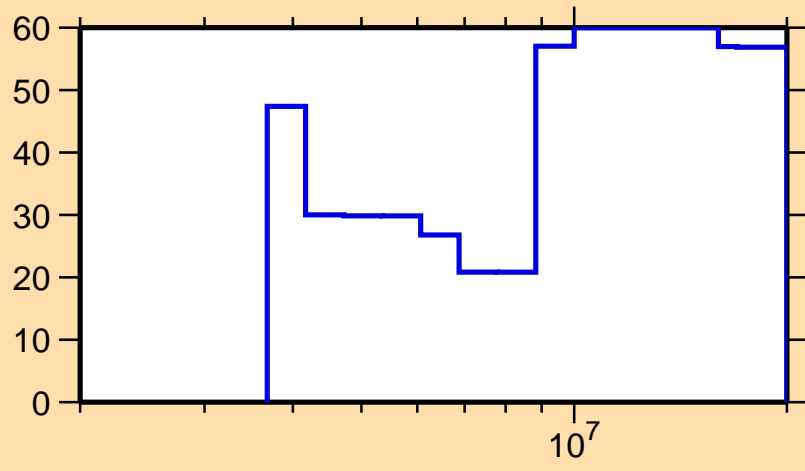
\Delta\sigma/\sigma vs. E for ^{169}\text{Gd}(n,2n)
