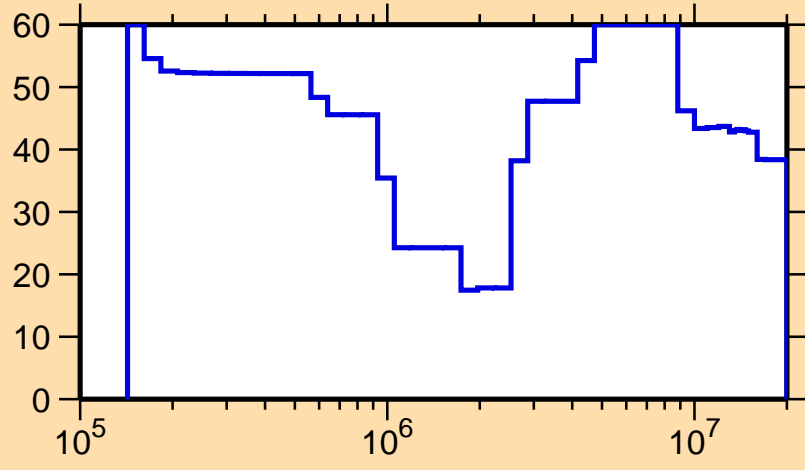
\Delta\sigma/\sigma vs. E for ^{169}\text{Gd}(n,\text{inel.})
