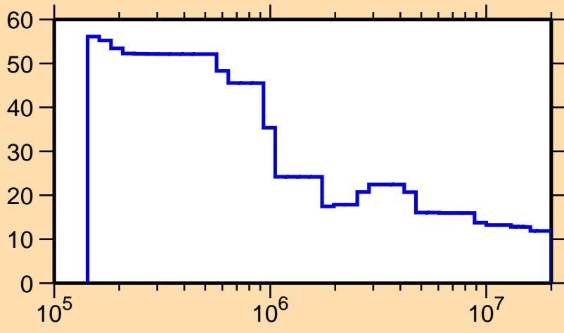
\Delta\sigma/\sigma vs. E for ^{169}\text{Gd}(n,\text{nonel.})
