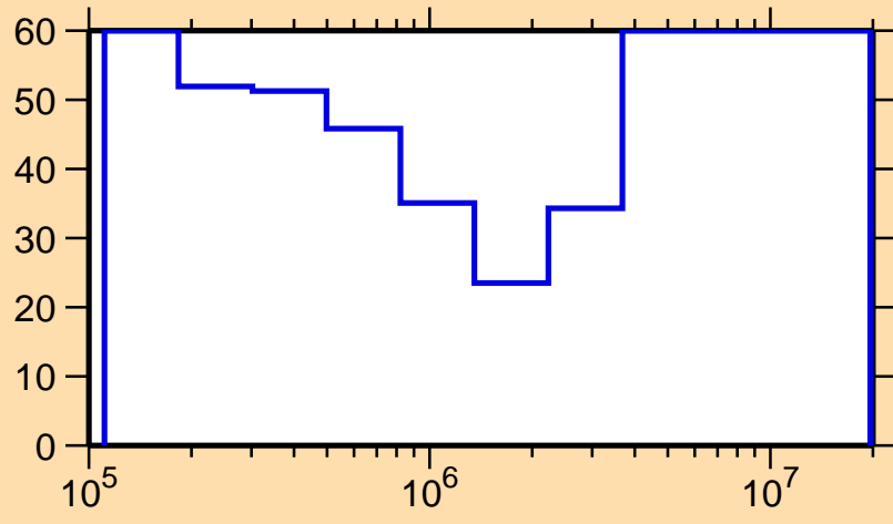
\Delta\sigma/\sigma vs. E for ^{169}\text{Gd}(n,n\text{cont.})
