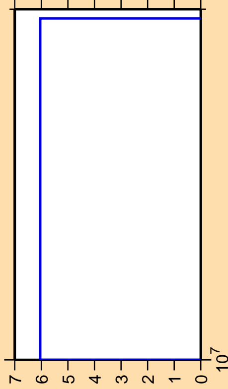
\Delta\sigma/\sigma vs. E for ^{169}\text{Gd}(n,2np)
