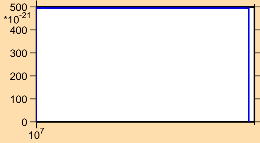
\sigma vs. E for ^{169}\text{Gd} (mt 11)
