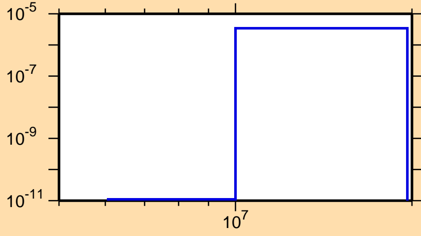
\sigma vs. E for ^{169}\text{Gd}(n,\alpha)
