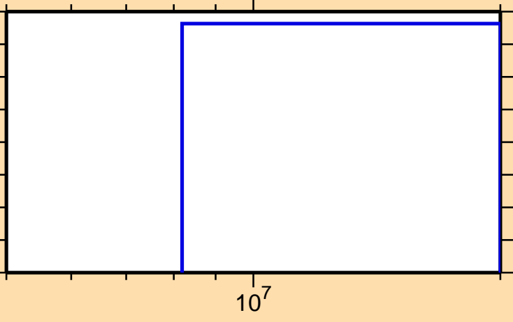
\sigma vs. E for ^{169}\text{Gd}(n,\text{nd})
