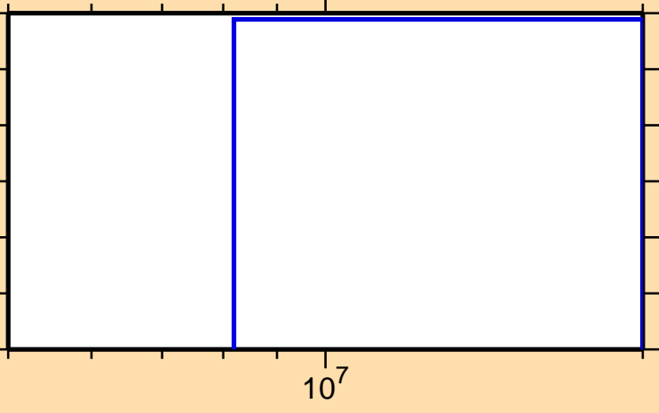
\sigma vs. E for ^{169}\text{Gd}(n,nt)
