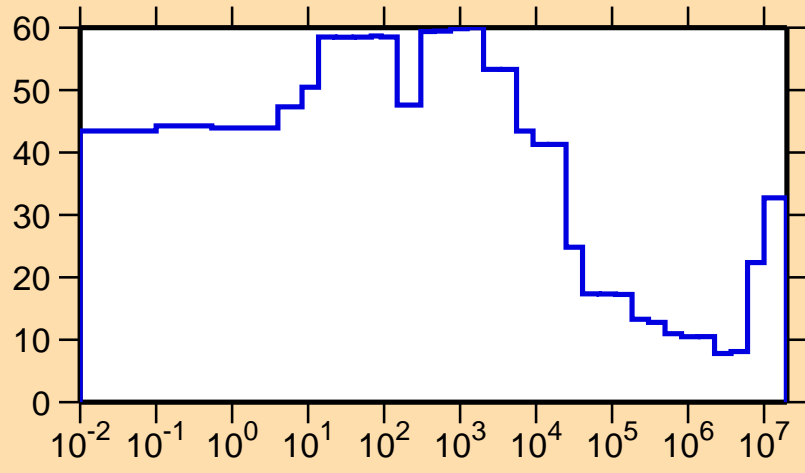
\Delta\sigma/\sigma vs. E for ^{64}\text{Ge}(n,p)
