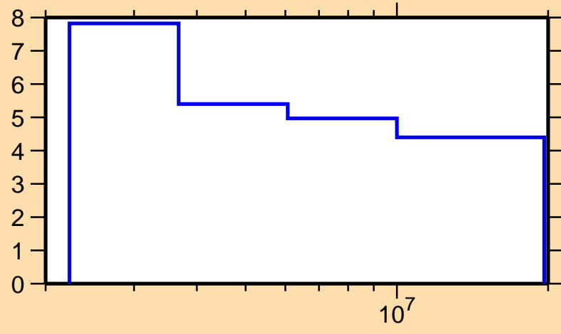
\Delta\sigma/\sigma vs. E for ^{64}\text{Ge}(n,n\text{onel.})
