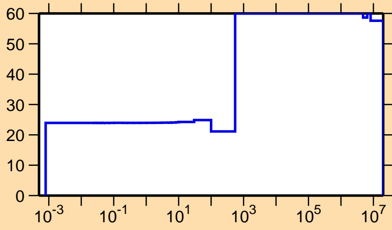
\Delta\sigma/\sigma vs. E for ^{64}\text{Ge}(n,\gamma)
