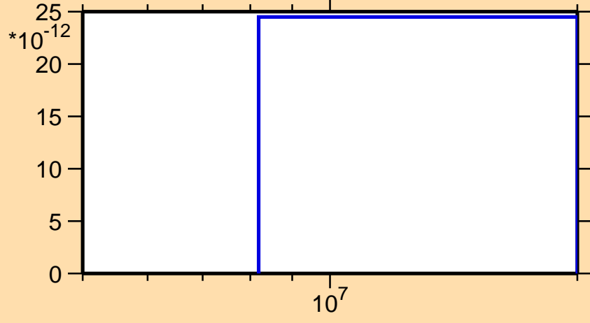
\sigma vs. E for ^{64}\text{Ge}(n,nd)
