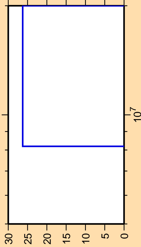
\Delta\sigma/\sigma vs. E for ^{64}\text{Ge}(n,nd)
