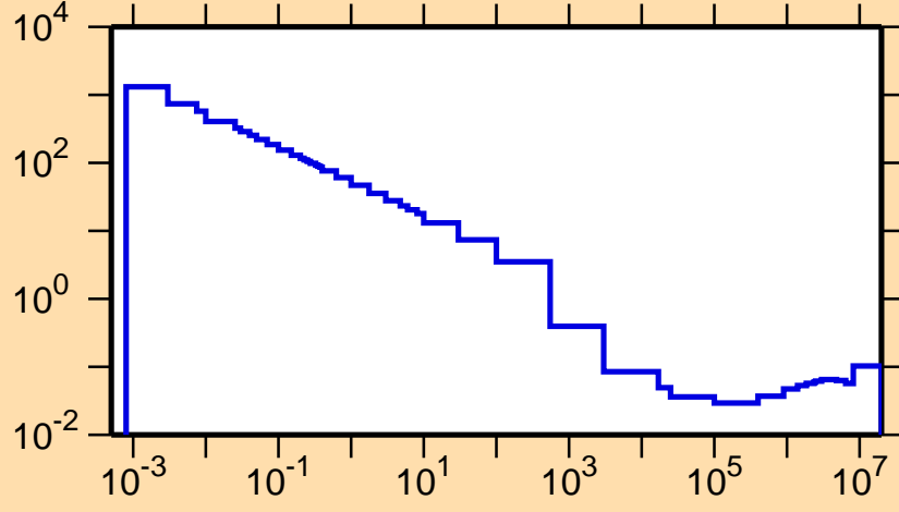
\sigma vs. E for ^{64}\text{Ge}(n,\alpha)
