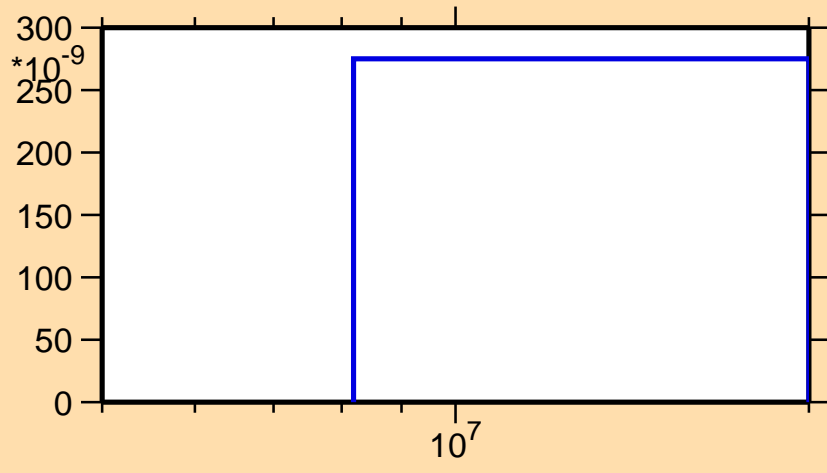
\sigma vs. E for ^{64}\text{Ge} (mt 45)
