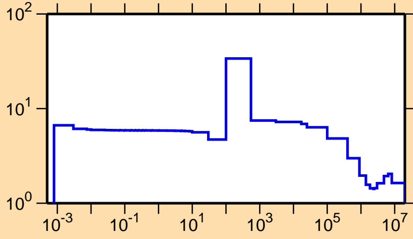
\sigma vs. E for ^{64}\text{Ge}(n,\text{el.})
