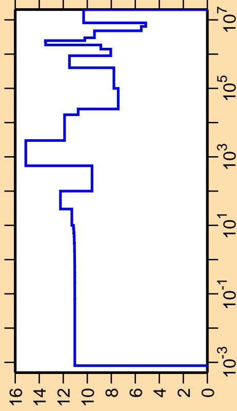
\Delta\sigma/\sigma vs. E for ^{64}\text{Ge}(n,\text{el.})
