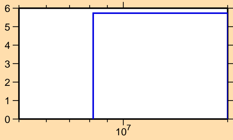
\Delta\sigma/\sigma vs. E for ^{64}\text{Ge}(n,\text{tot.})
