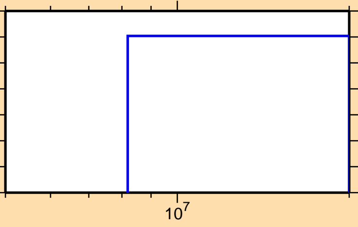
\sigma vs. E for ^{64}\text{Ge}(n,2n)
