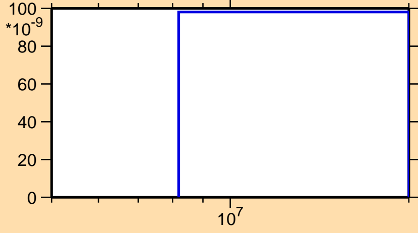
\sigma vs. E for ^{64}\text{Ge}(\text{mt117})
