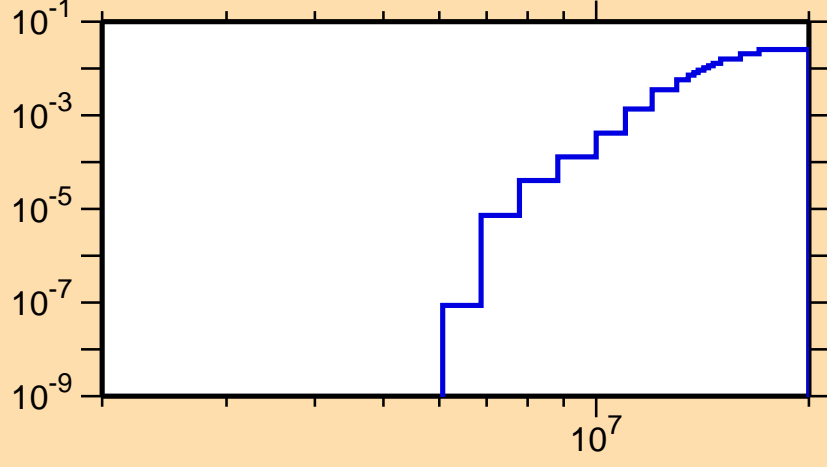
\sigma vs. E for ^{65}\text{Ge}(n,n\alpha)
