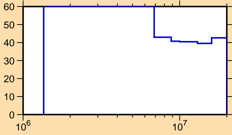
\Delta\sigma/\sigma vs. E for ^{65}\text{Ge}(n,n\text{cont.})
