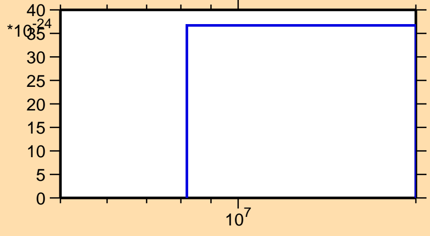
\sigma vs. E for ^{65}\text{Ge}(n,nt)
