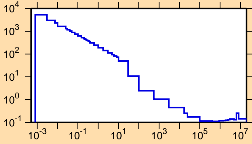
\sigma vs. E for ^{65}\text{Ge}(n,\alpha)
