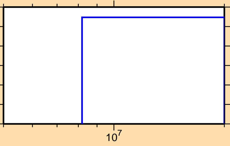
\sigma vs. E for ^{65}\text{Ge}(n,2np)
