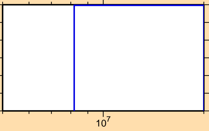
\sigma vs. E for ^{65}\text{Ge}(n,2n)
