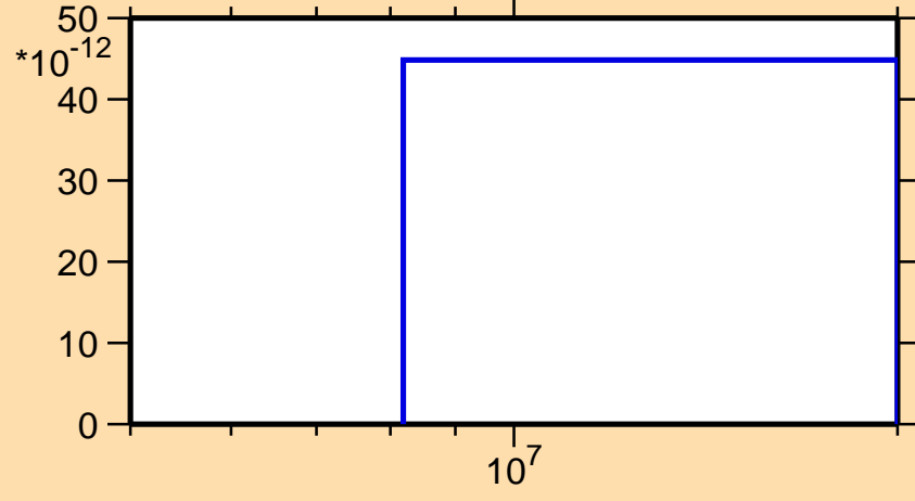
\sigma vs. E for ^{65}\text{Ge}(n,2n\alpha)
