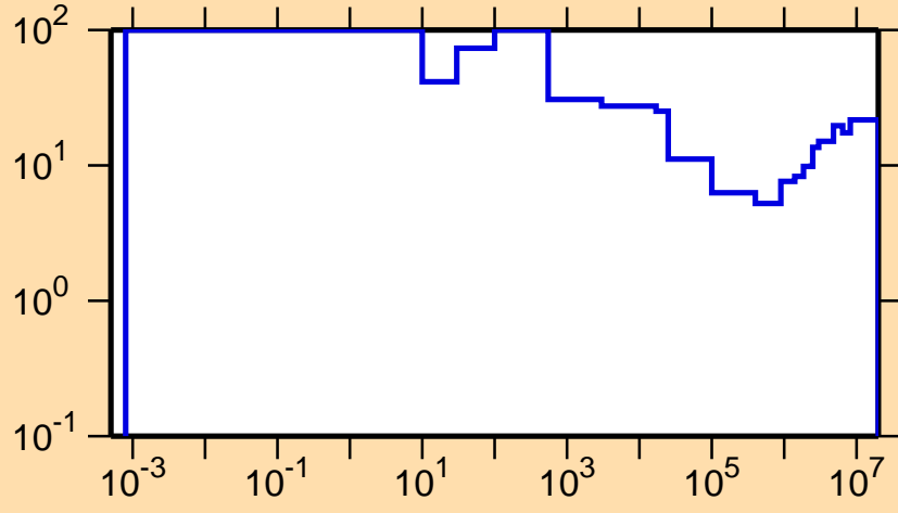
\Delta\sigma/\sigma vs. E for ^{65}\text{Ge}(n,p)
