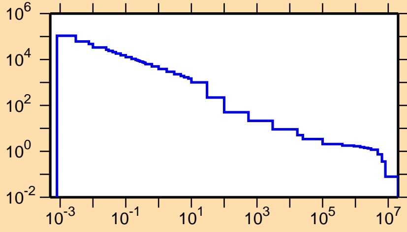
\sigma vs. E for ^{65}\text{Ge}(n,p)
