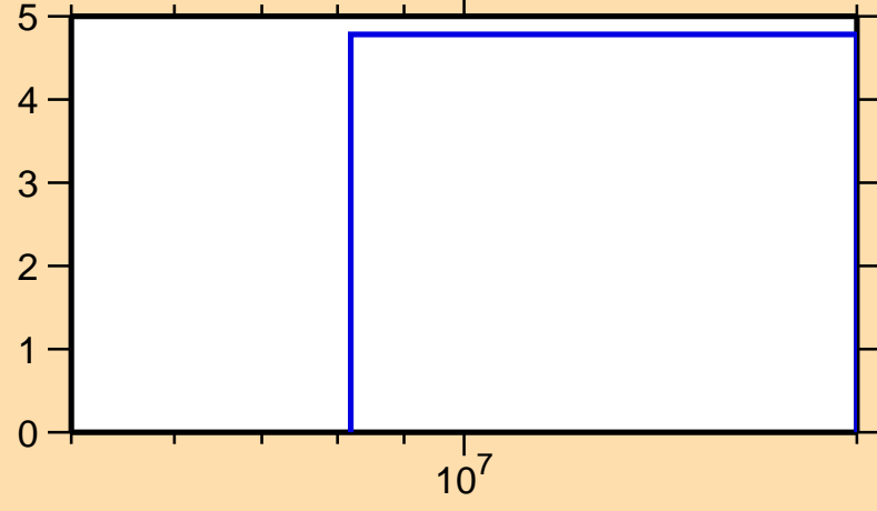
\Delta\sigma/\sigma vs. E for ^{65}\text{Ge}(n,\text{tot.})
