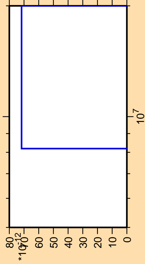
\Delta\sigma/\sigma vs. E for ^{65}\text{Ge}(n,nt)
