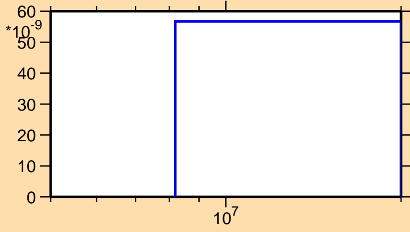
\sigma vs. E for ^{65}\text{Ge}(\text{mt } 34)
