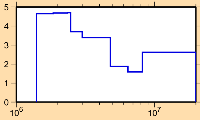
\Delta\sigma/\sigma vs. E for ^{65}\text{Ge}(n,\text{nonel.})
