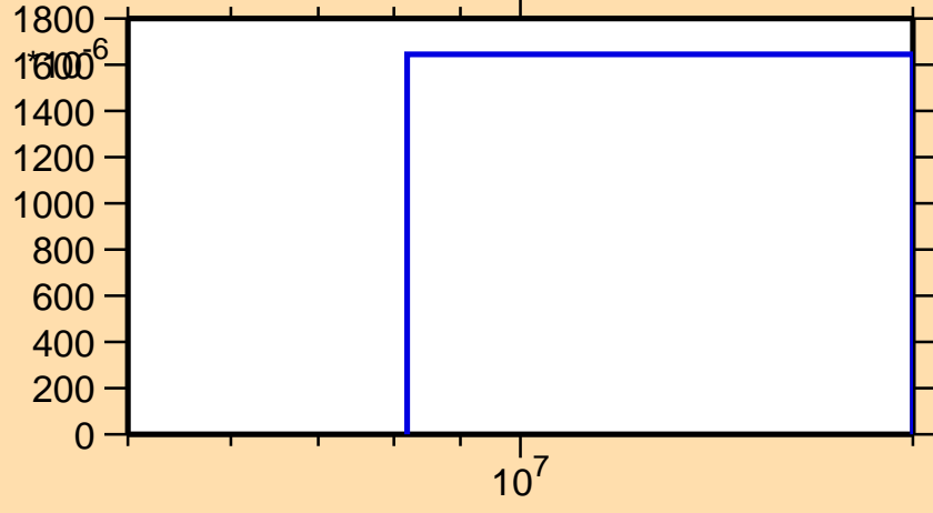
\sigma vs. E for ^{65}\text{Ge}(n,\text{pd})
