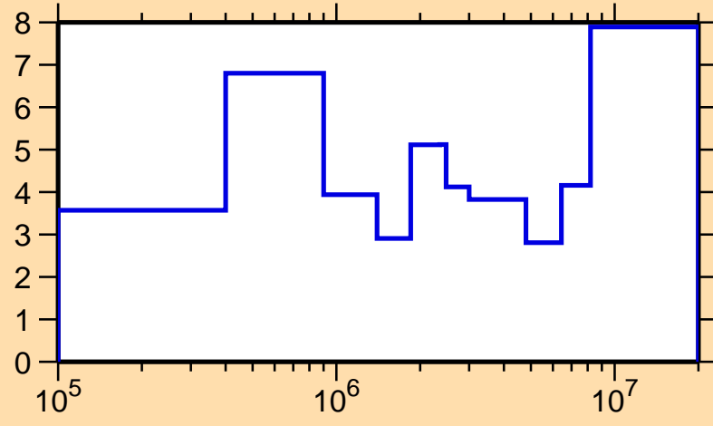
\Delta\sigma/\sigma vs. E for ^{65}\text{Ge}(n,\text{el.})
