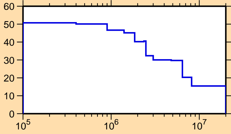
\Delta\sigma/\sigma vs. E for ^{65}\text{Ge}(n,n_1)
