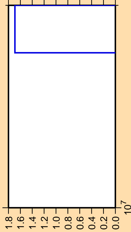
\Delta\sigma/\sigma vs. E for ^{66}\text{Ge}(n,2n\alpha)
