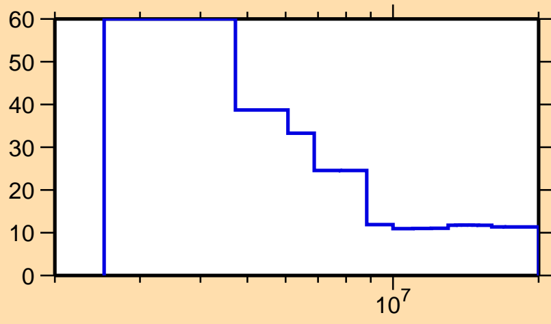
\Delta\sigma/\sigma vs. E for ^{66}\text{Ge}(n,n\text{cont.})
