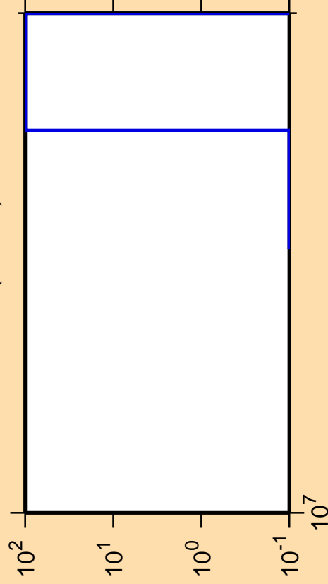
\Delta\sigma/\sigma vs. E for ^{66}\text{Ge} (mt 34)
