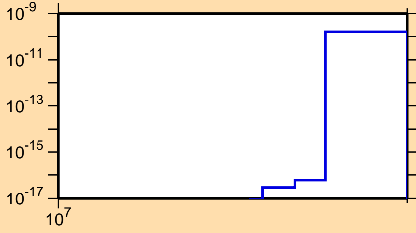
\sigma vs. E for ^{66}\text{Ge} (mt 34)
