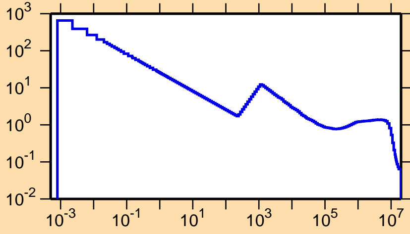
\sigma vs. E for ^{66}\text{Ge}(n,p)
