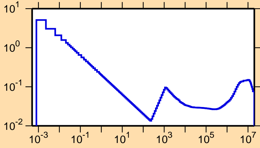
\sigma vs. E for ^{66}\text{Ge}(n,\alpha)
