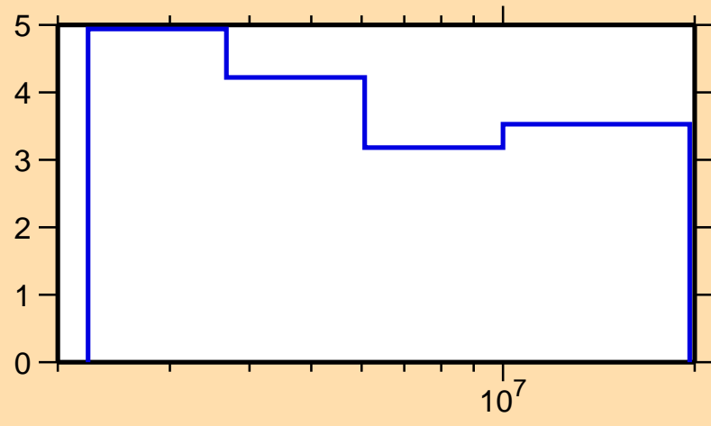
\Delta\sigma/\sigma vs. E for ^{67}\text{Ge}(n,n\text{inel.})
