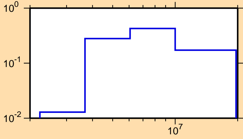
\sigma vs. E for ^{67}\text{Ge}(n,n\text{cont.})
