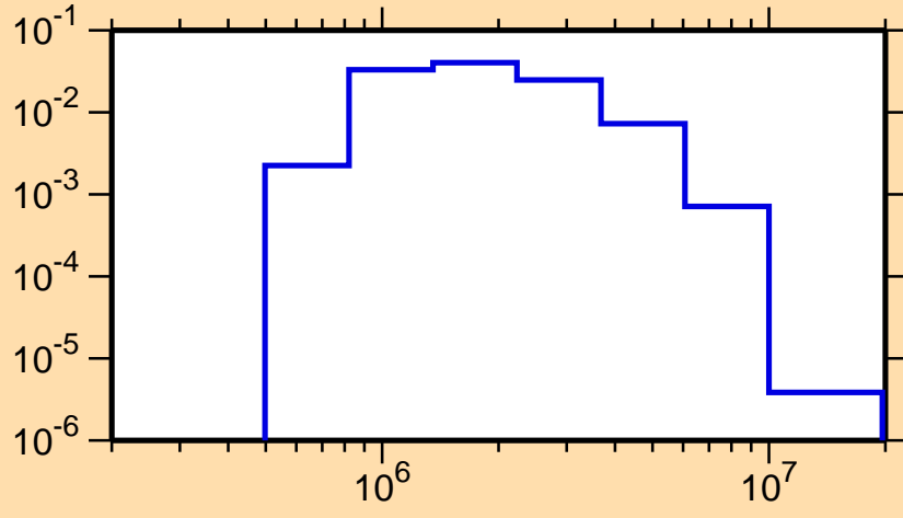
\sigma vs. E for ^{67}\text{Ge}(n,n_4)
