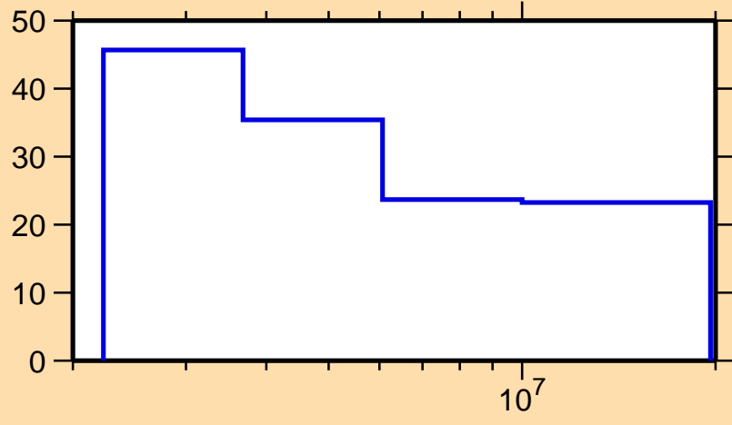
\Delta\sigma/\sigma vs. E for ^{67}\text{Ge}(n,ncont.)
