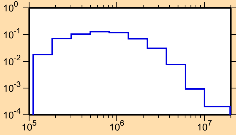
\sigma vs. E for ^{67}\text{Ge}(n,n_2)
