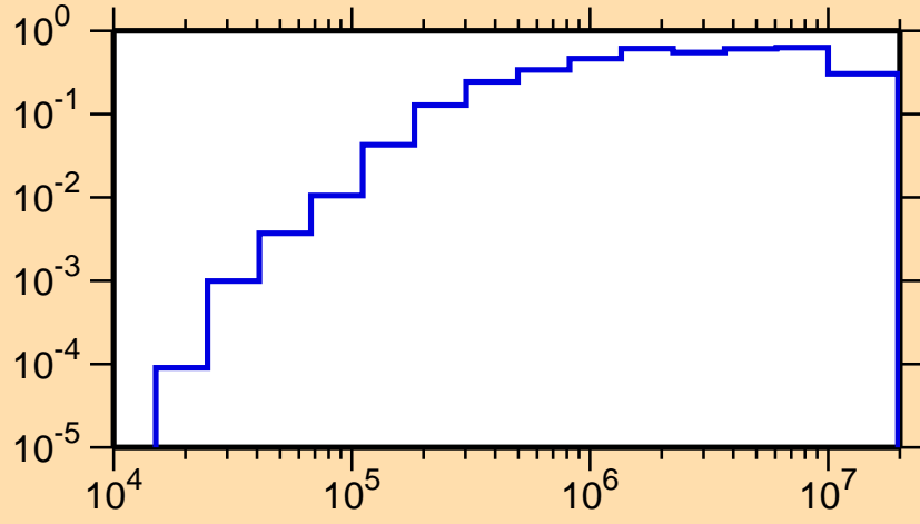
\sigma vs. E for ^{67}\text{Ge}(n,\text{inel.})
