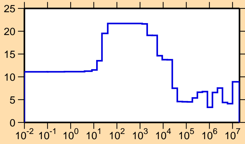
\Delta\sigma/\sigma vs. E for ^{67}\text{Ge}(n,el.)
