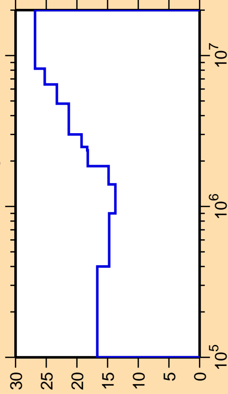
\Delta\sigma/\sigma vs. E for ^{67}\text{Ge}(n,n_3)
