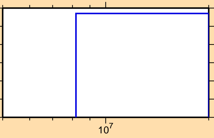
\sigma vs. E for ^{67}\text{Ge}(\text{mt117})
