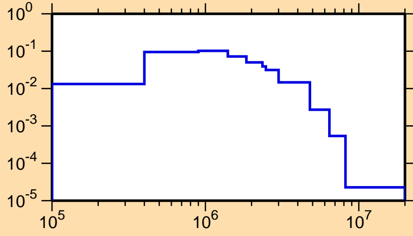
\sigma vs. E for ^{67}\text{Ge}(n,n_3)
