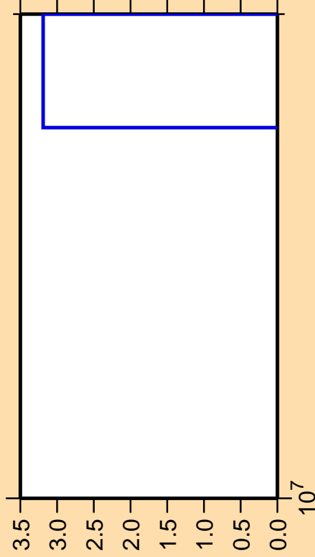
\Delta\sigma/\sigma vs. E for ^{68}\text{Ge}(n,2np)
