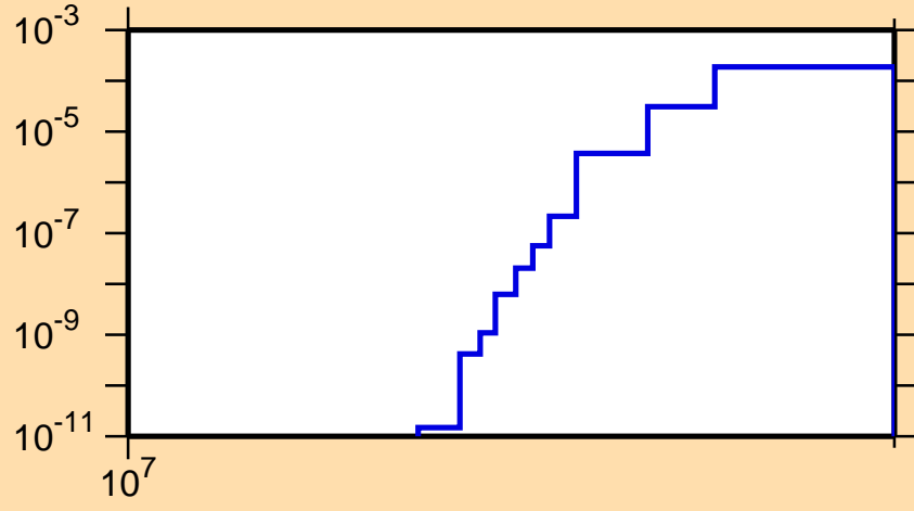
\sigma vs. E for ^{68}\text{Ge}(n,\text{pd})
