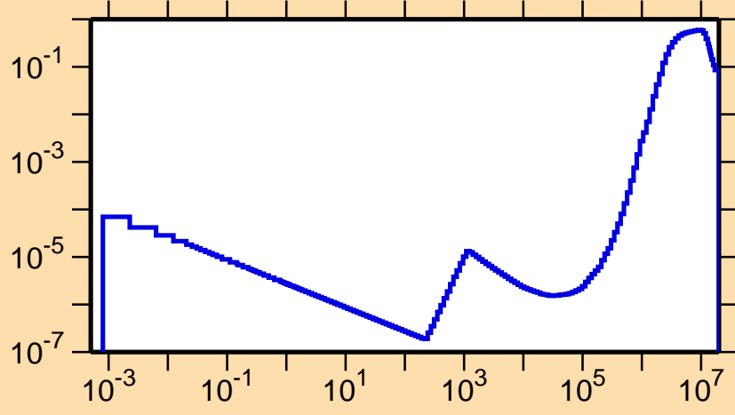
\sigma vs. E for ^{68}\text{Ge}(n,p)
