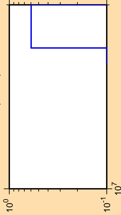
\Delta\sigma/\sigma vs. E for ^{68}\text{Ge} (mt 34)
