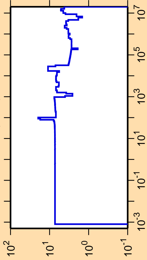
\Delta\sigma/\sigma vs. E for ^{68}\text{Ge}(n,\text{el.})
