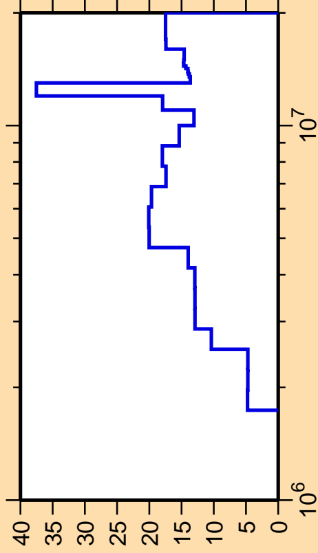
\Delta\sigma/\sigma vs. E for ^{68}\text{Ge}(n,n_2)
