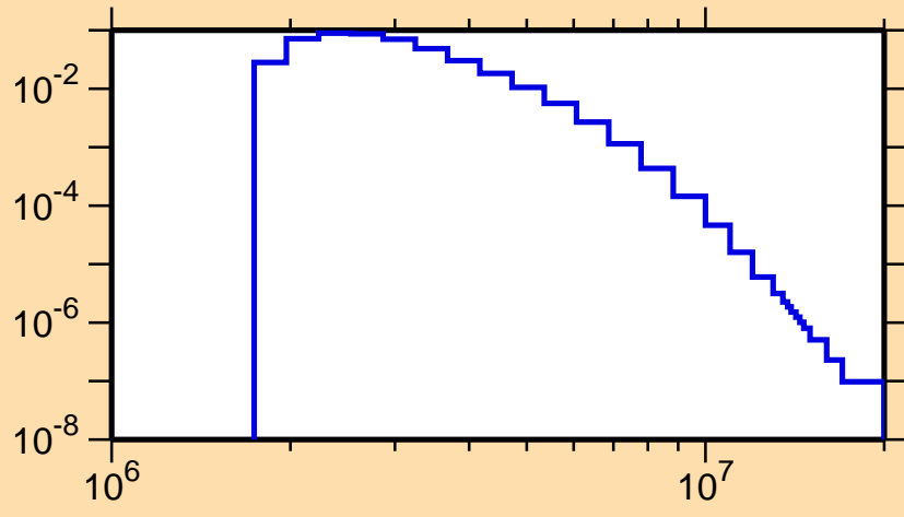
\sigma vs. E for ^{68}\text{Ge}(n,n_2)
