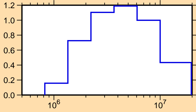
\sigma vs. E for ^{68}\text{Ge}(n,\text{inel.})
