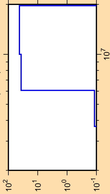
\Delta\sigma/\sigma vs. E for ^{68}\text{Ge}(n,n\alpha)
