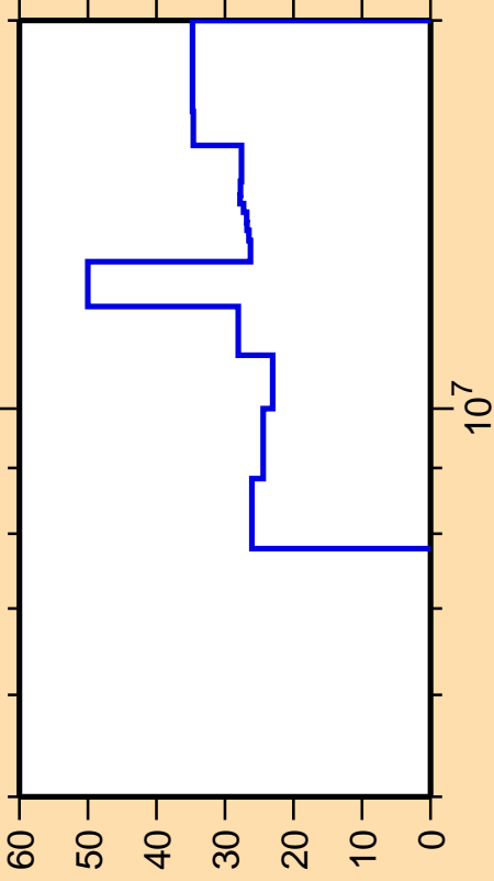
\Delta\sigma/\sigma vs. E for ^{69}\text{Ge}(n,n_1)
