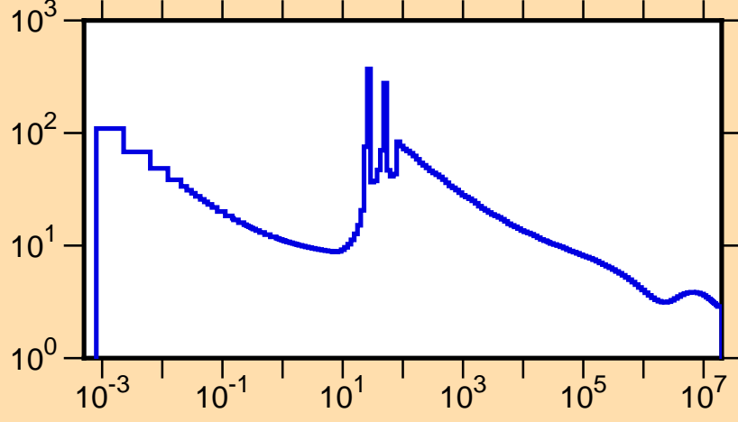
\sigma vs. E for ^{69}\text{Ge}(n,\text{tot.})
