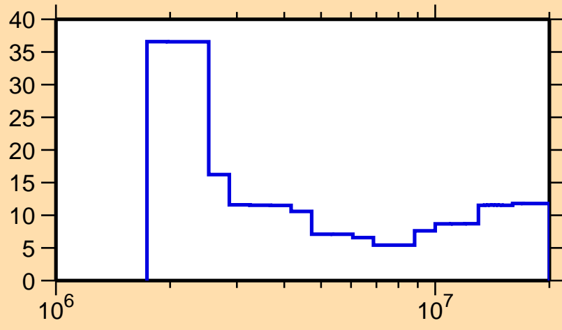
\Delta\sigma/\sigma vs. E for ^{69}\text{Ge}(n,ncont.)
