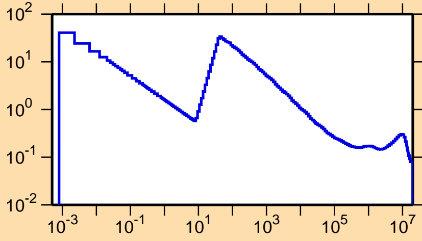
\sigma vs. E for ^{69}\text{Ge}(n,p)
