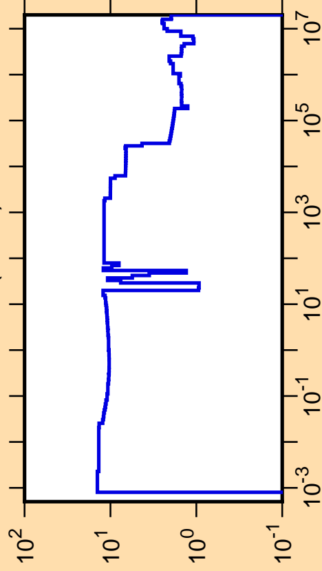
\Delta\sigma/\sigma vs. E for ^{69}\text{Ge}(n,\text{tot.})
